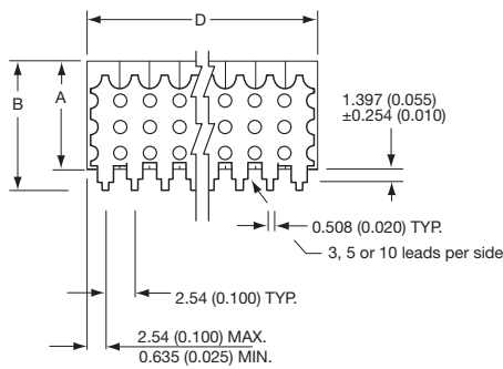
“J” STYLE LEADS
