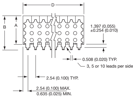
“L” STYLE LEADS
