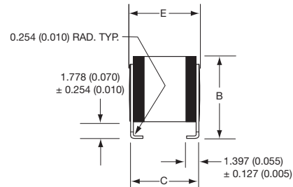
“N” STYLE LEADS
