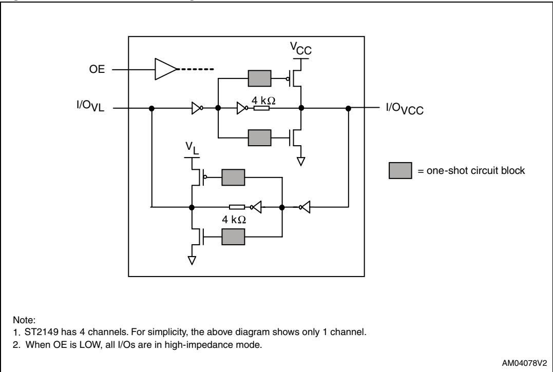
Figure 3. ST2149 block diagram
