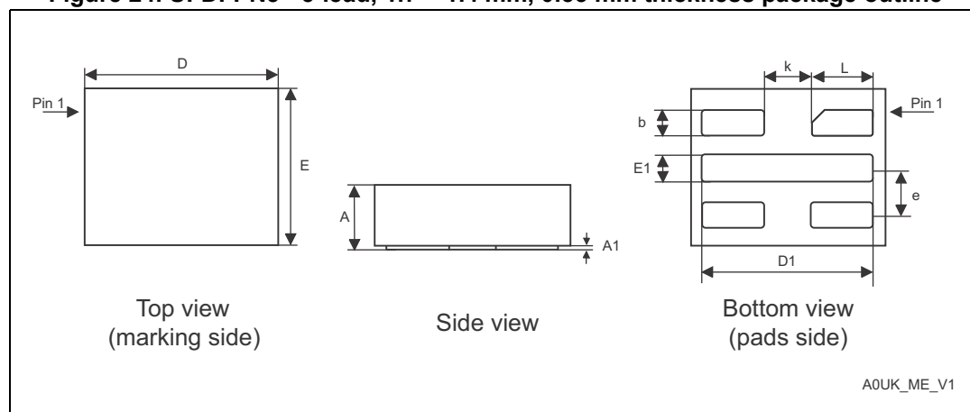
Figure 24. UFDFPN5 - 5-lead, 1.7 × 1.4 mm, 0.55 mm thickness package outline
