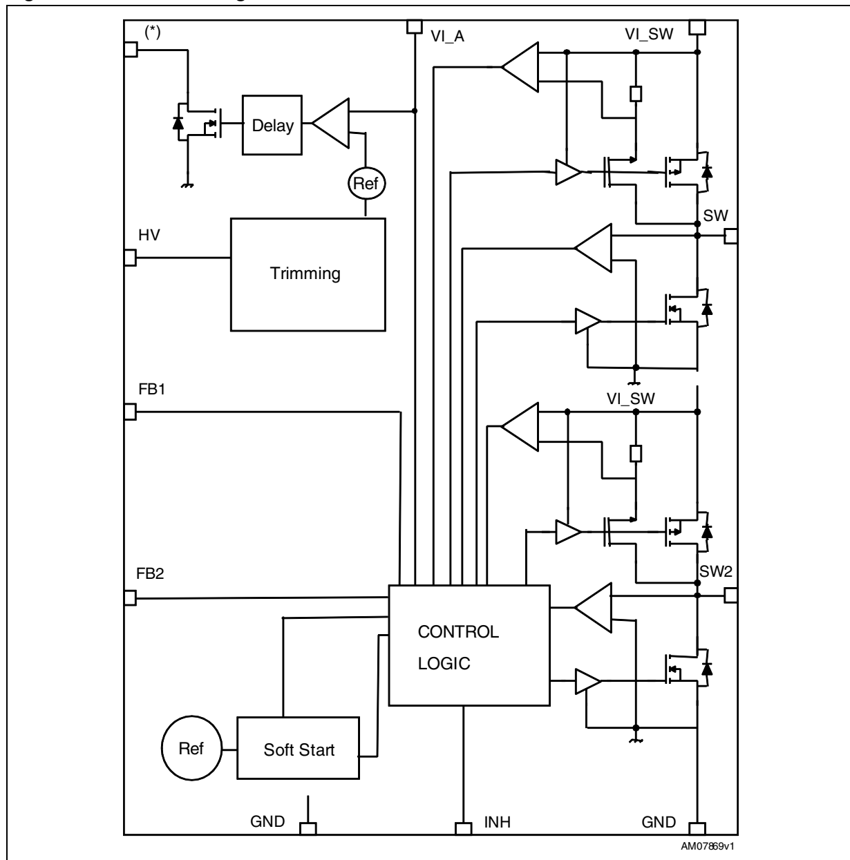
Figure 1. Schematic diagram
