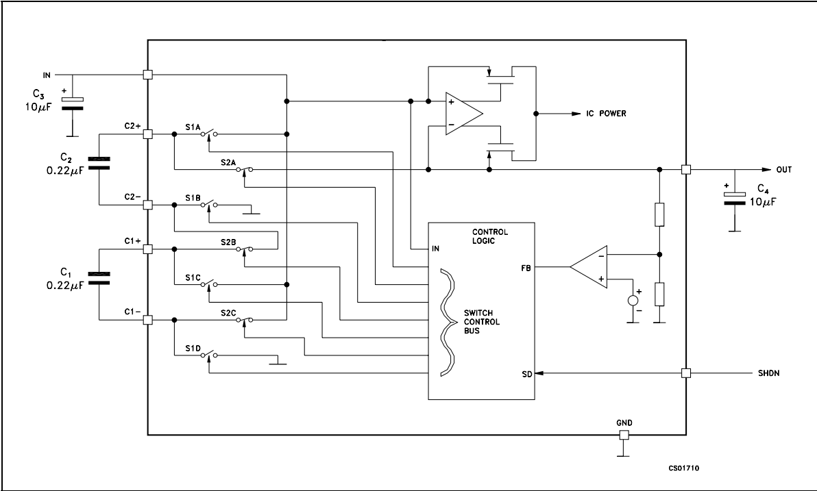
Figure 1. Schematic diagram
