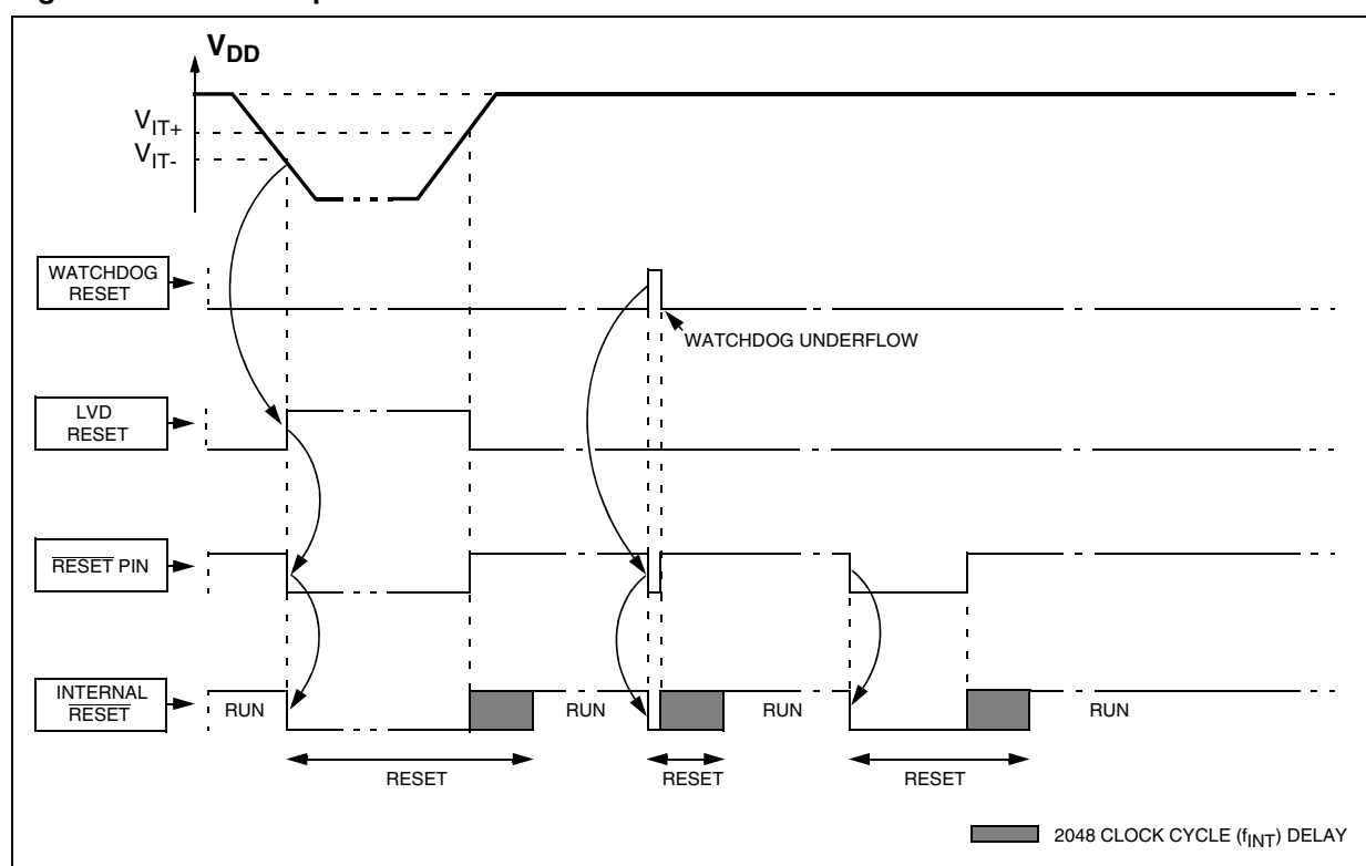
Figure 13. RESET Sequence
