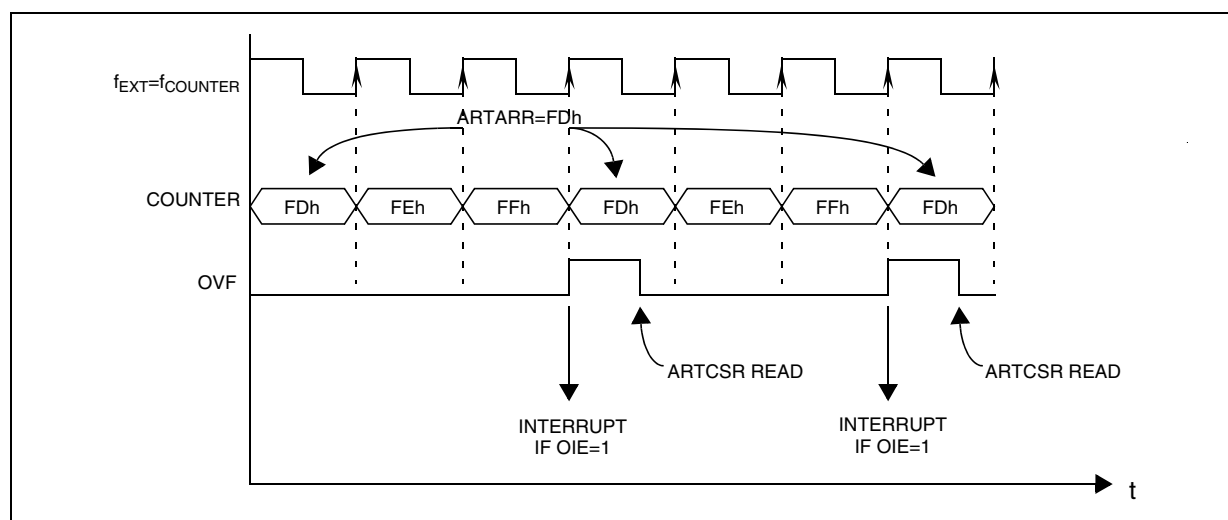
Figure 41. External Event Detector Example (3 counts)
