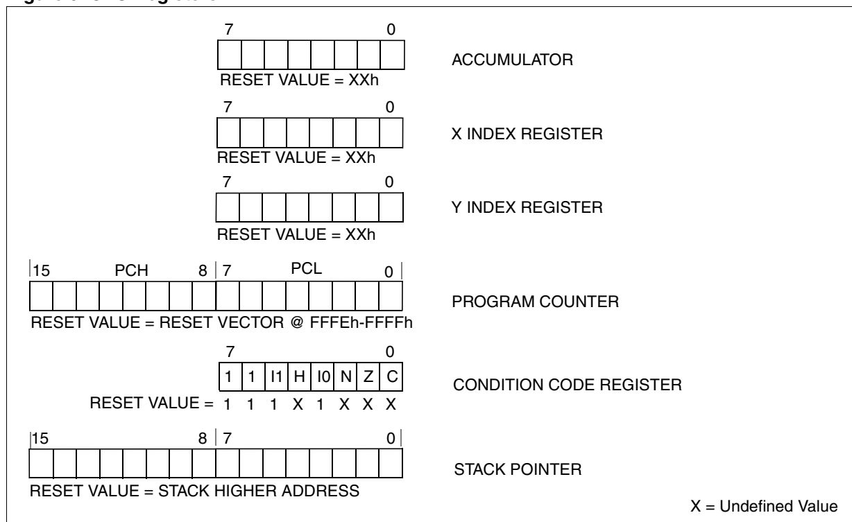
Figure 9. CPU Registers
