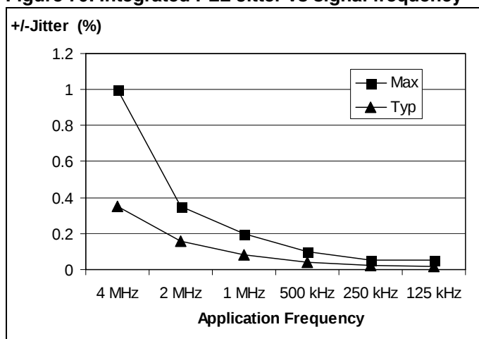
Figure 79. Integrated PLL Jitter vs signal frequency 1
