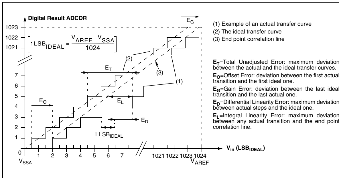
Figure 99. ADC Accuracy Characteristics
