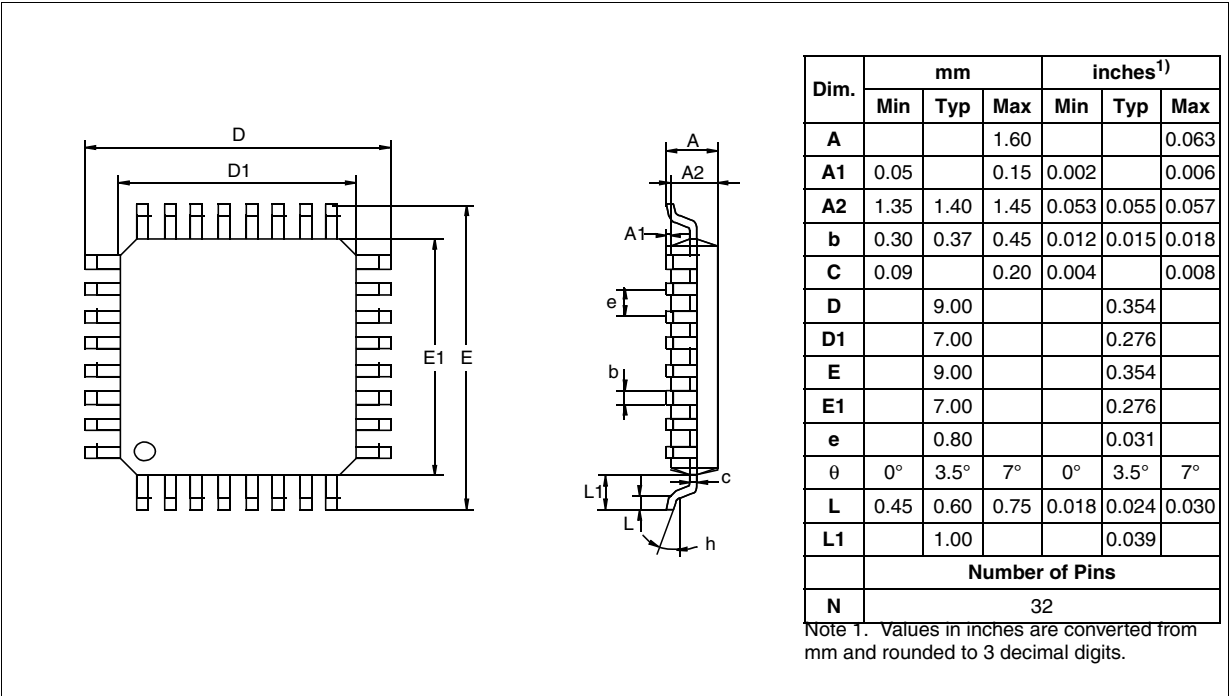
Figure 106. 32-Pin Low Profile Quad Flat Package
