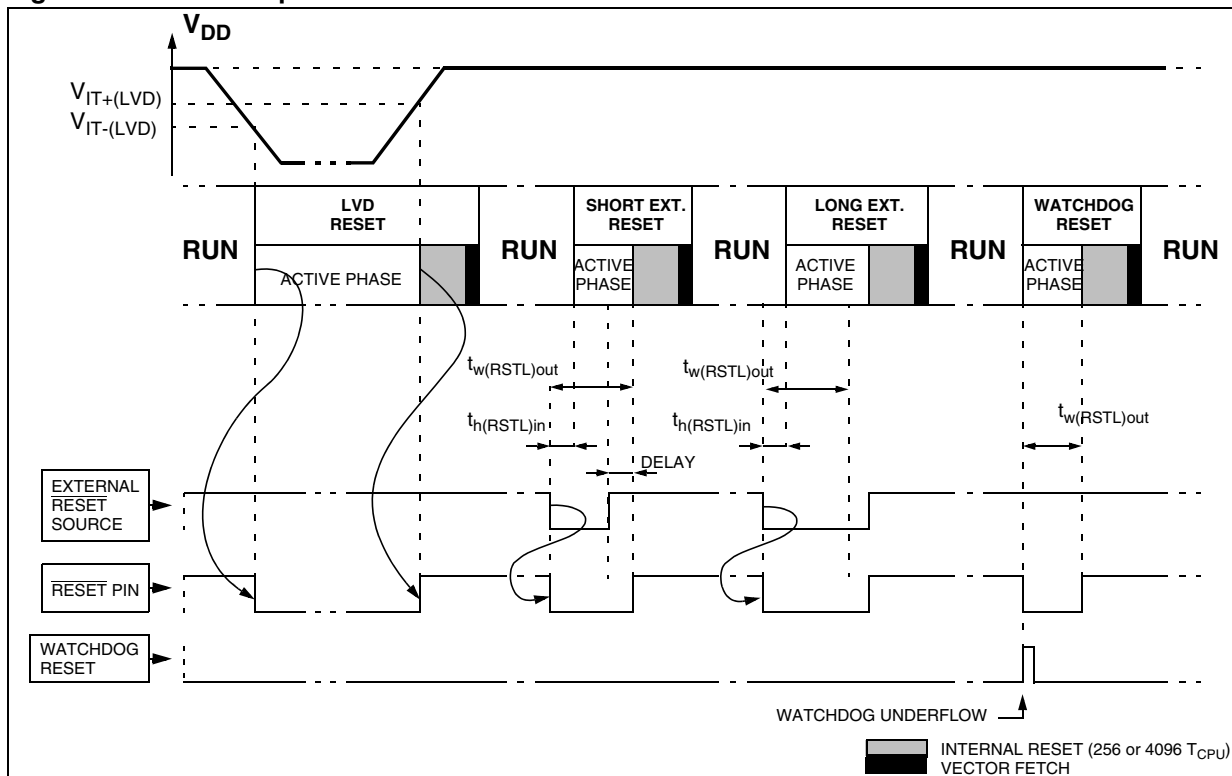
Figure 16. RESET Sequences
