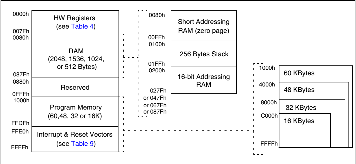
Figure 6. Memory Map
