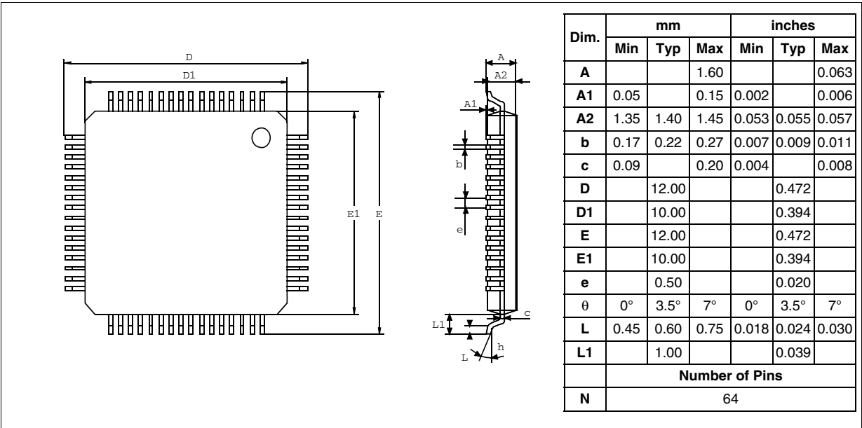
Figure 101. 64-Pin Low Profile Quad Flat Package 10 x10
