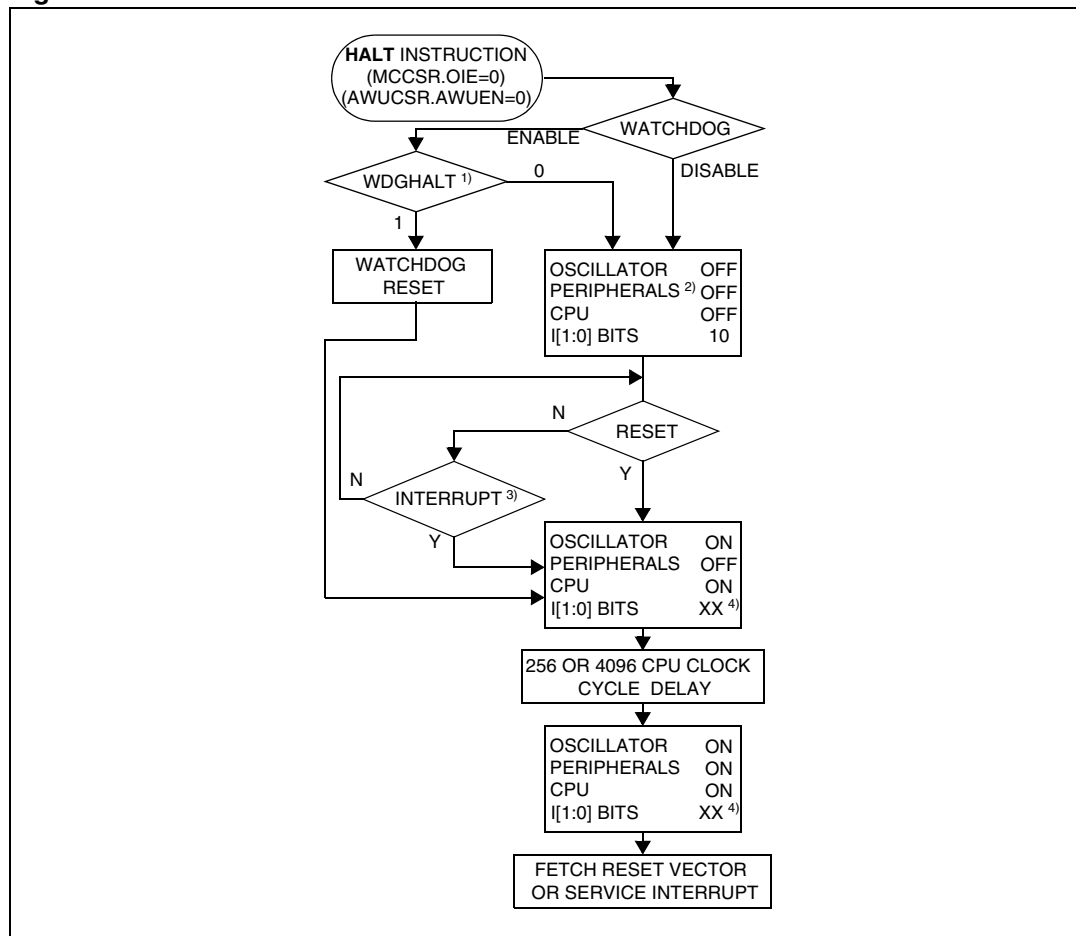
Figure 26. HALT mode flow-chart
