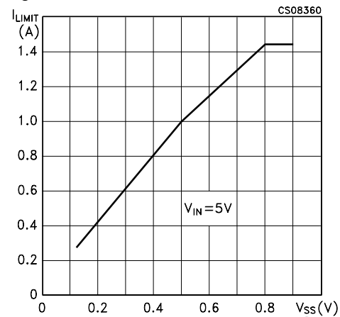
Figure 10 : Switch Current Limit vs Soft Start Voltage
