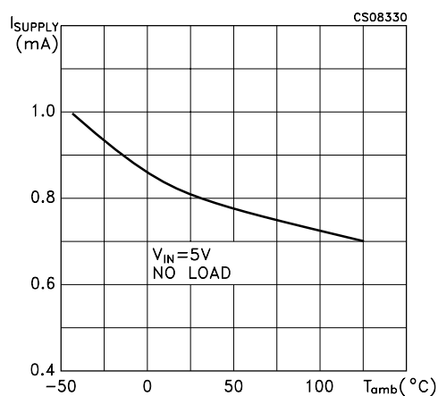
Figure 6 : Supply Current vs Temperature
