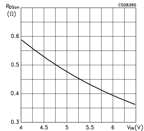
Figure 12 : LX On Resistance vs Input Voltage
