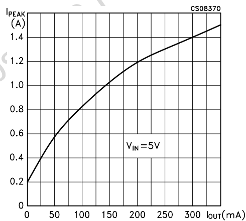
Figure 9 : Peak Inductor Current vs Output Current
