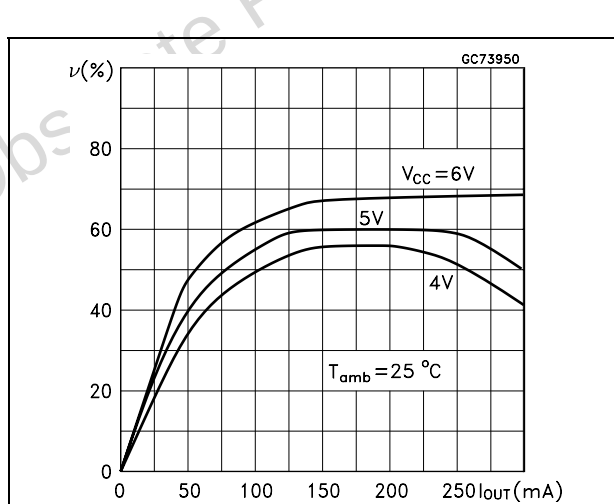
Figure 9. Efficiency vs load current
