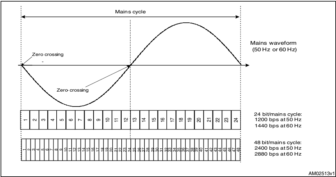
Figure 13. Bit timing
