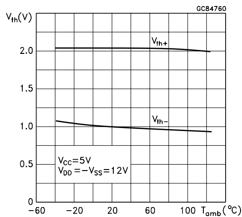
Figure 13 : Receiver Threshold vs Temperature
