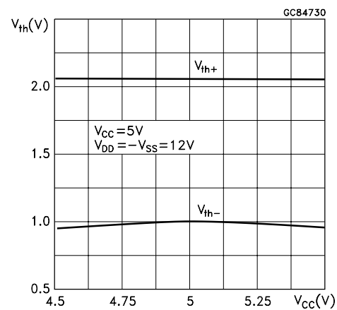
Figure 14 : Receiver Threshold vs Supply Voltage
