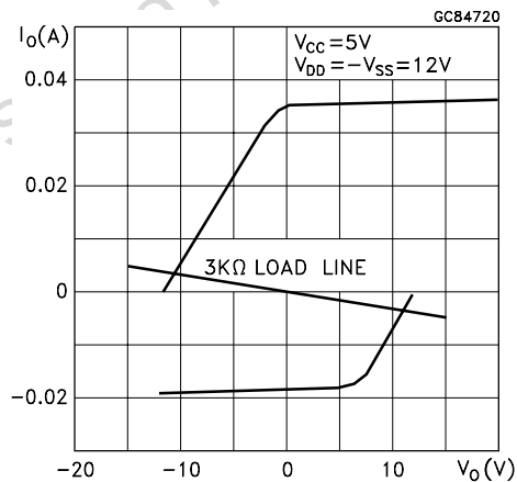
Figure 10 : Driver Output Current vs Output Voltage
