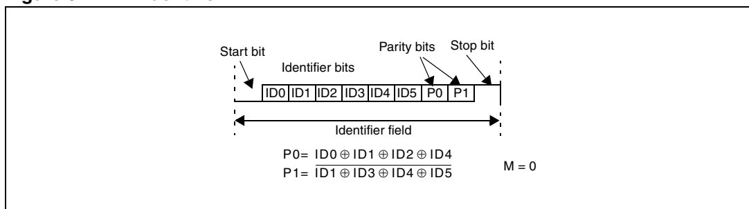
Figure 62. LIN identifier
