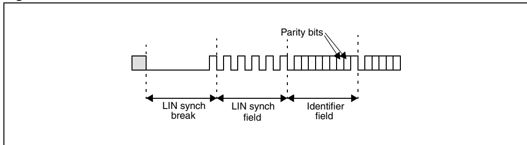
Figure 61. LIN header
