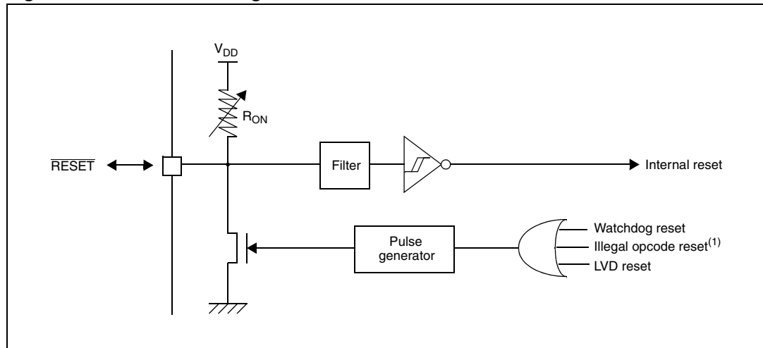
Figure 16. Reset block diagram
