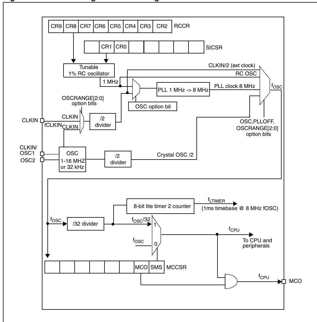
Figure 13. Clock management block diagram
