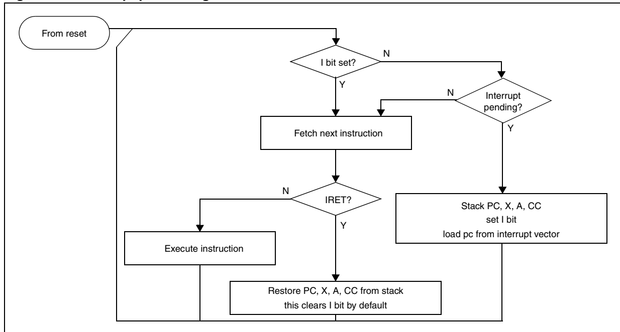
Figure 21. Interrupt processing flowchart
