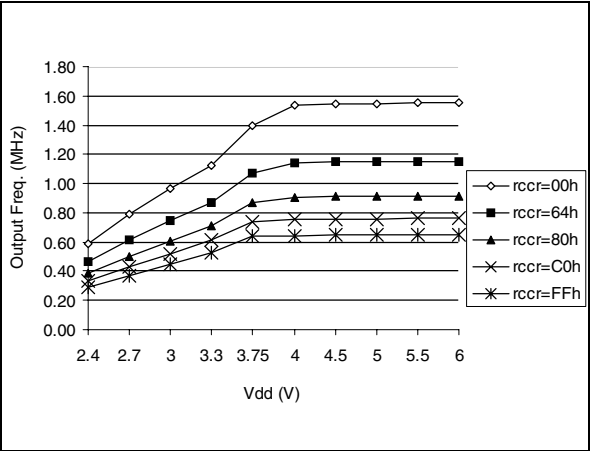
Figure 52. RC Osc Freq vs V_{DD} and RCCR Value
