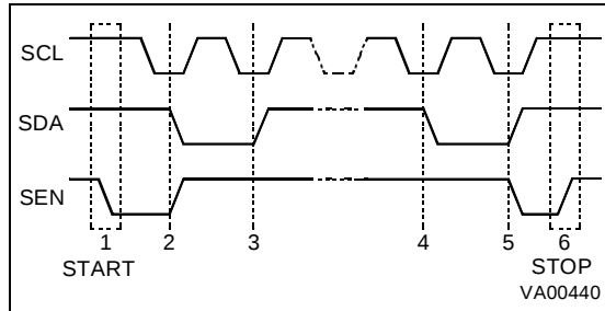
Figure 71. Mixed S-bus and I 2 C-bus System
