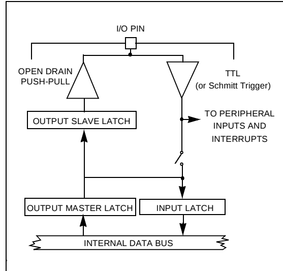
Figure 52. Output Configuration
