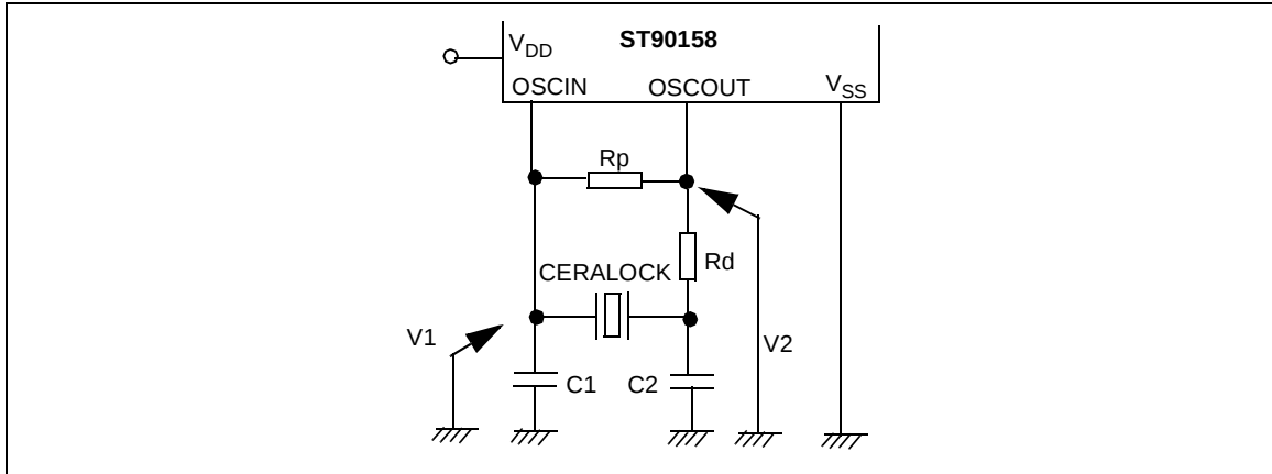
Figure 40. Test circuit
