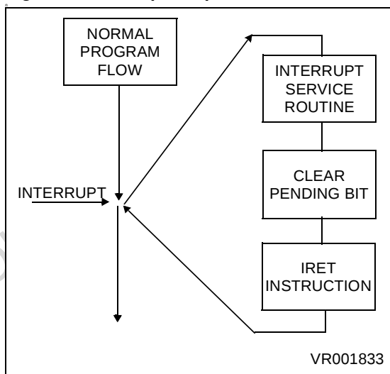
Figure 19. Interrupt Response
