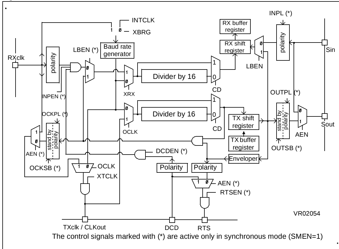
Figure 77. SCI -M Functional Schematic
