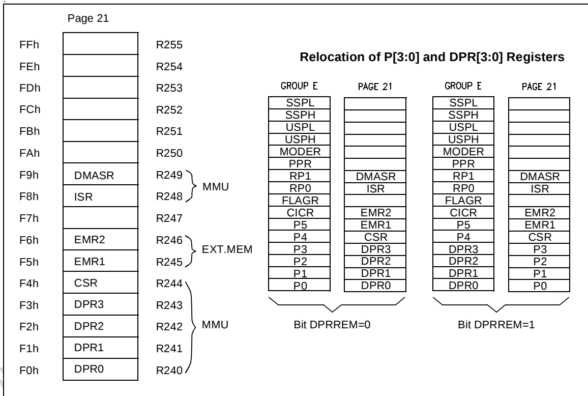
Figure 43. Page 21 Registers
