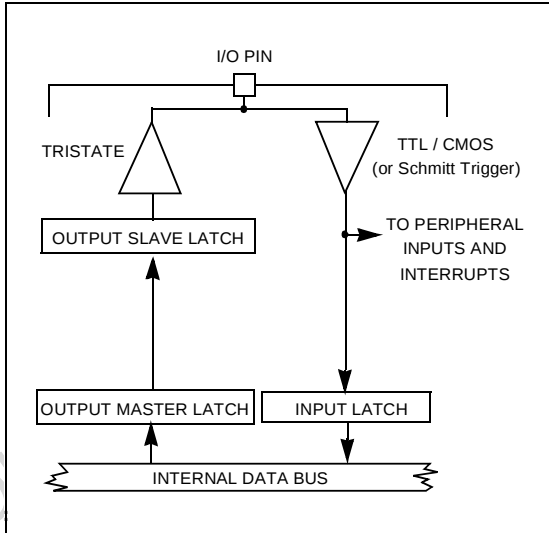
Figure 51. Input Configuration
