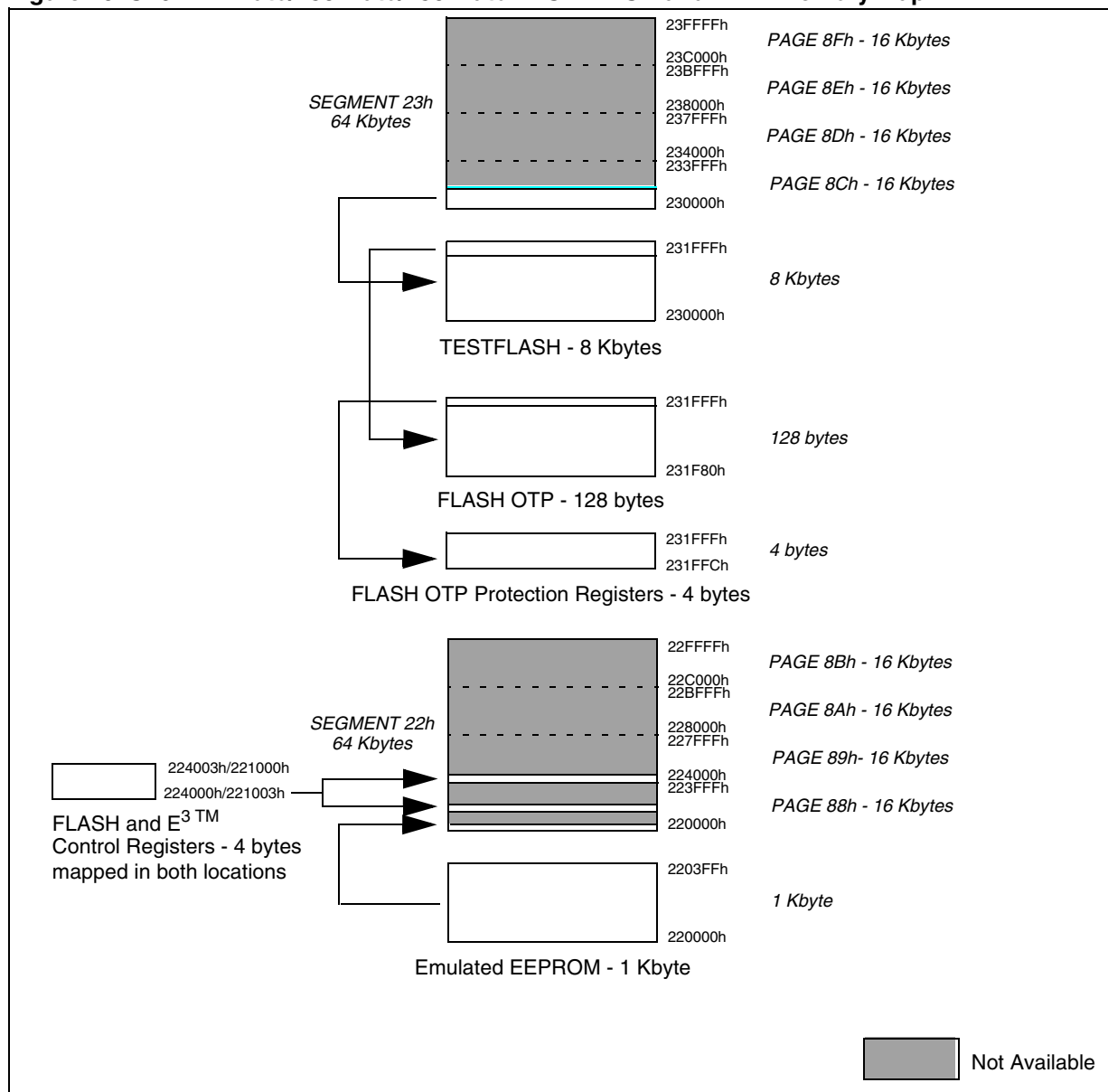
Figure 40. ST92124-Auto/150-Auto/250-Auto TESTFLASH and E 3 ™ Memory Map
