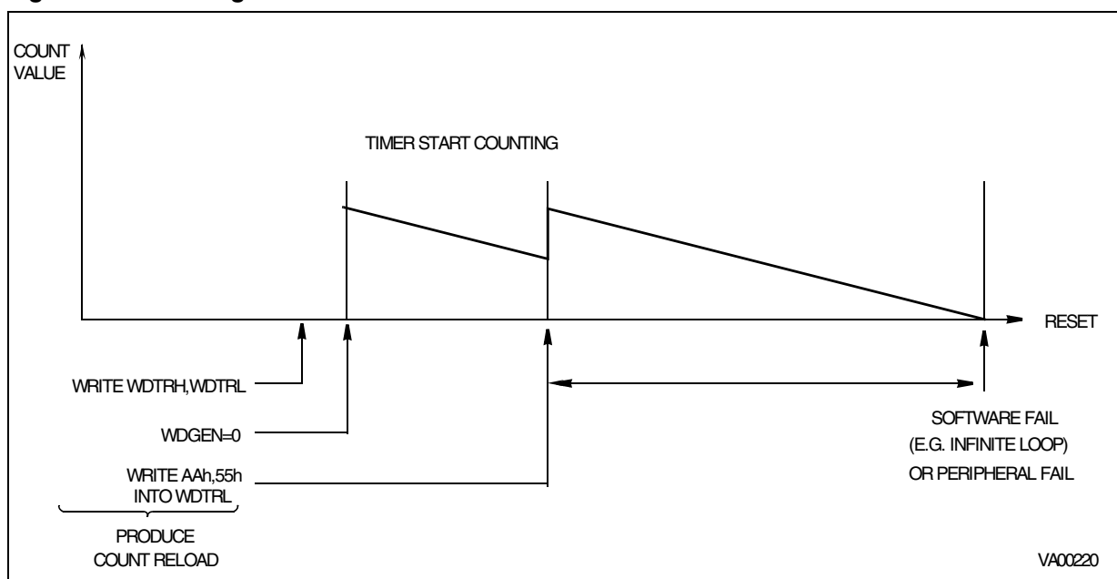
Figure 88. Watchdog Timer Mode
