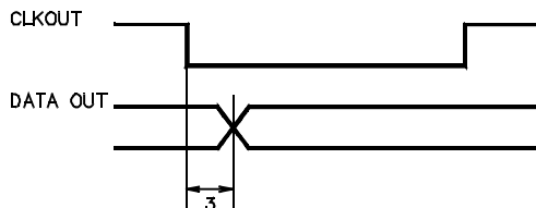
FIG 3: TRANSMISSION WITH CLKOUT 1X MODE
