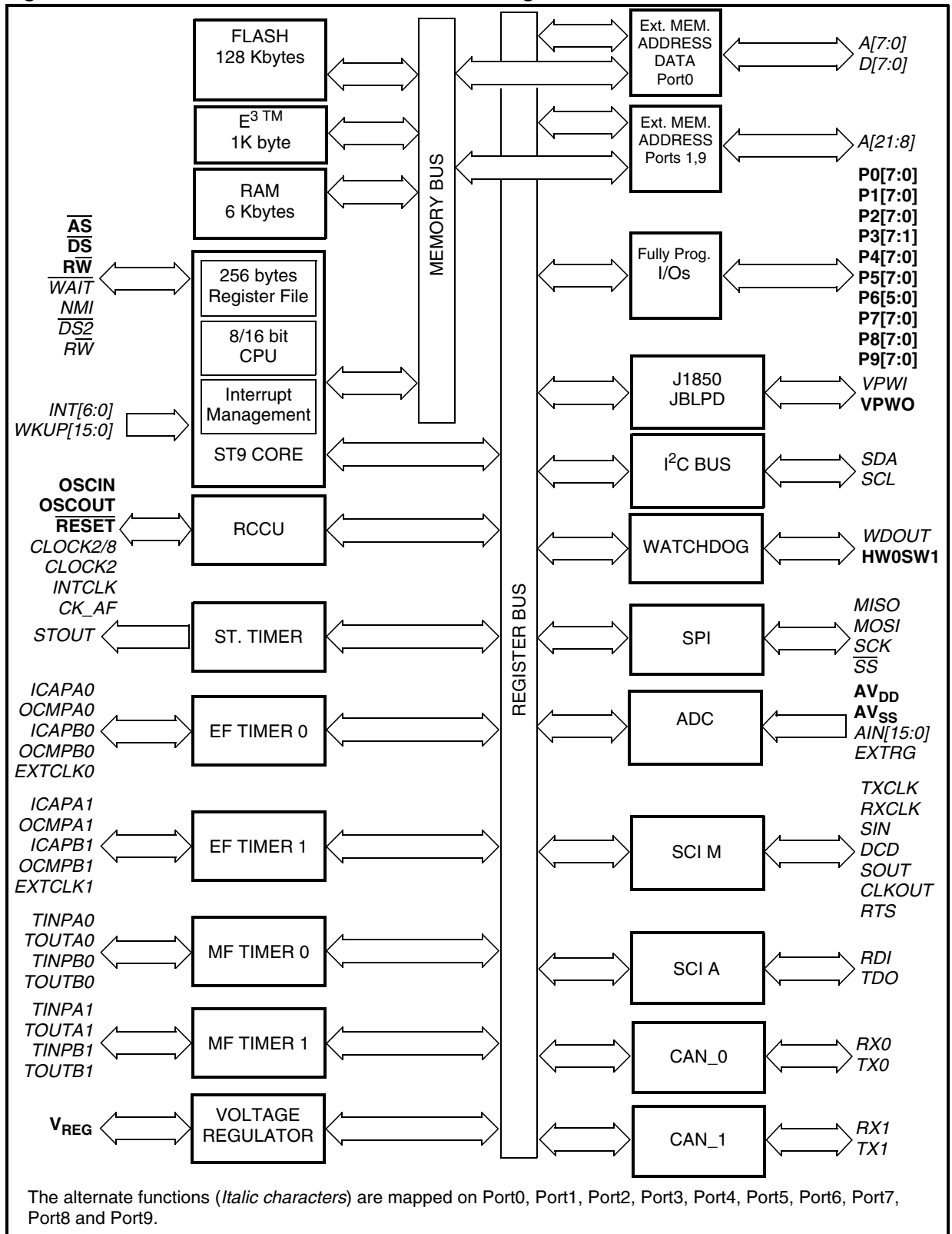
Figure 4. ST92150JDV1-Auto: Architectural Block Diagram
