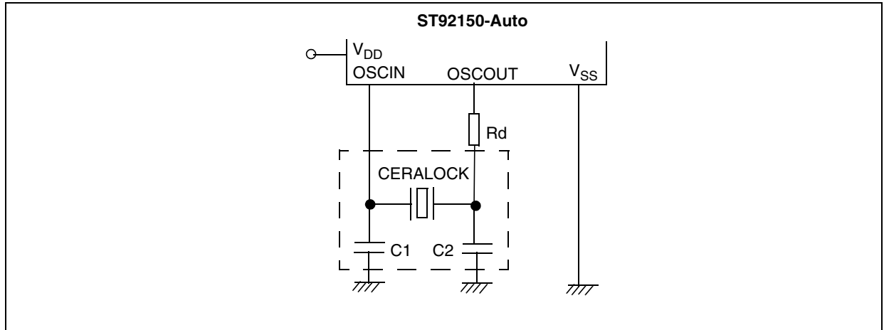
Figure 69. Test Circuit
