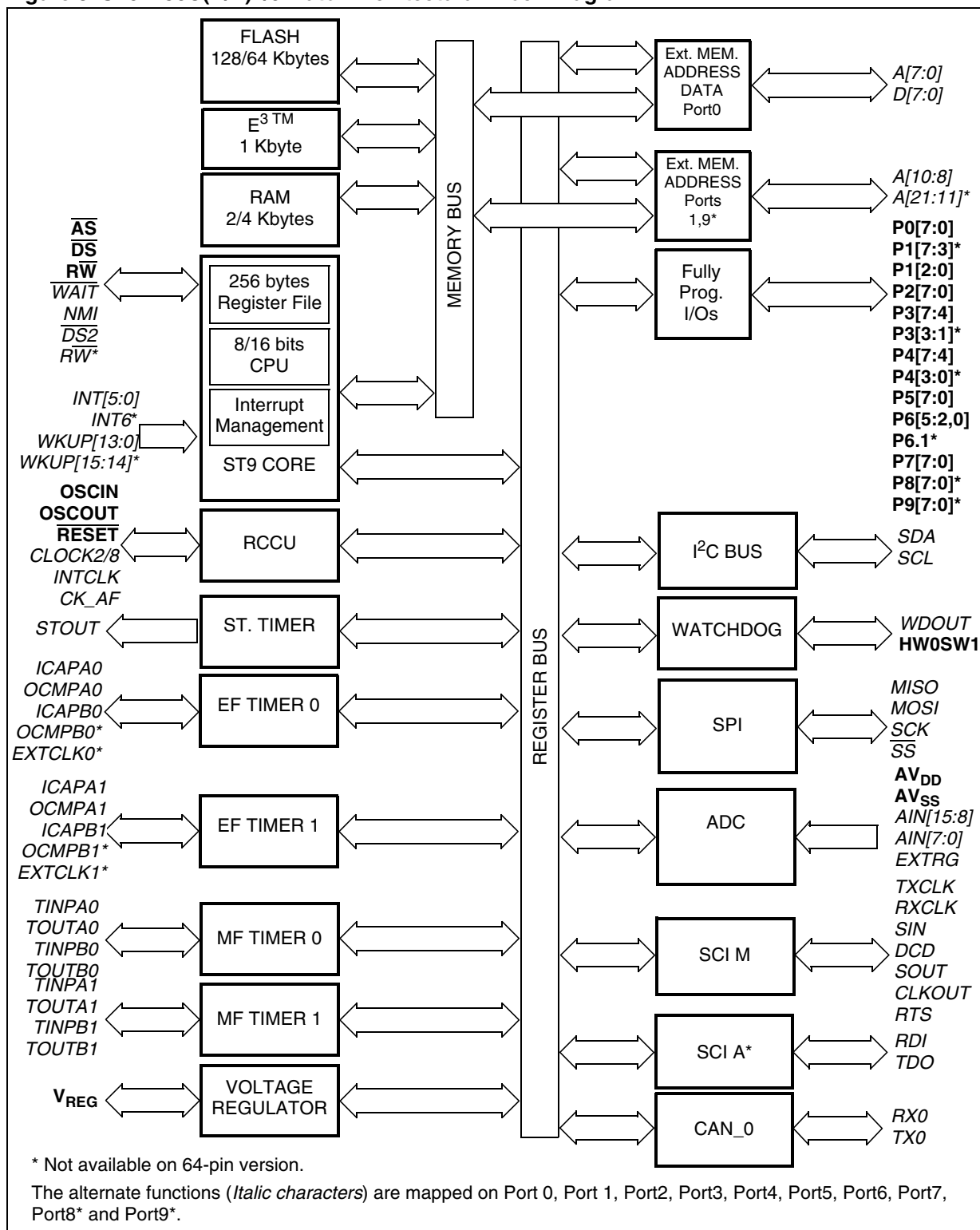
Figure 3. ST92150C(R/V)1/9-Auto: Architectural Block Diagram
