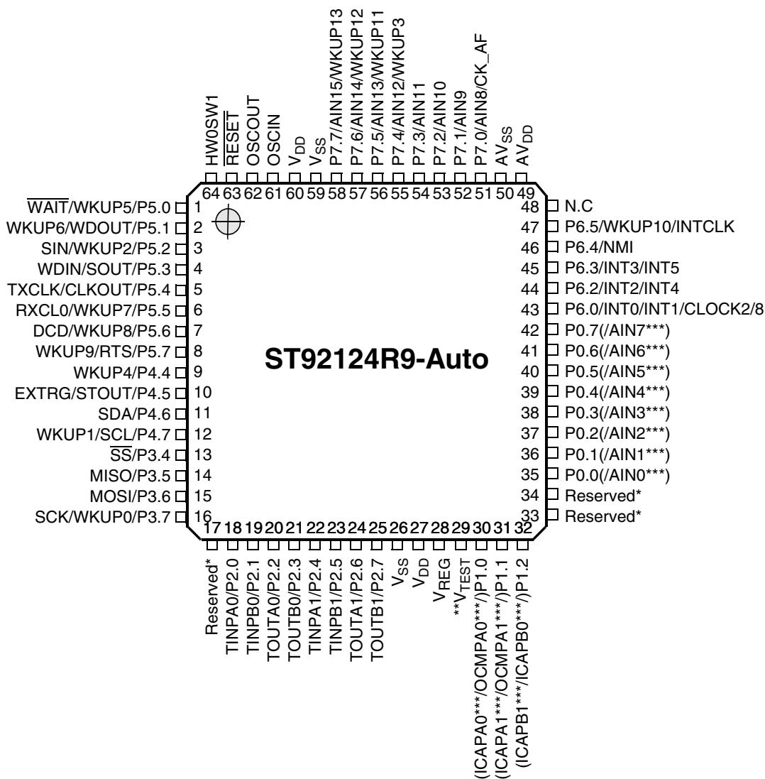
Figure 6. ST92124R9-Auto: Pin Configuration (Top-view LQFP64)
