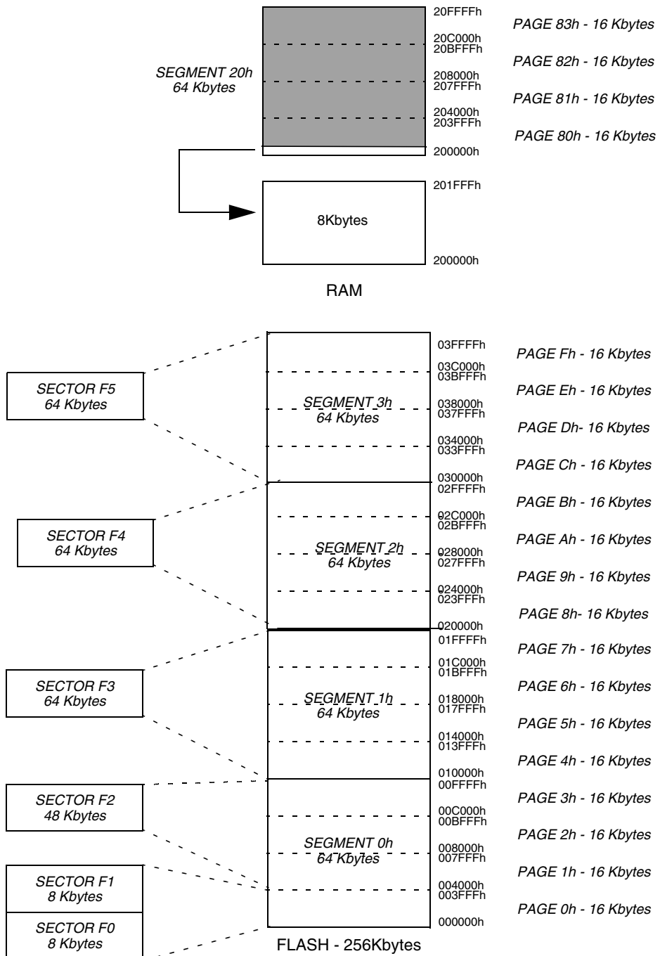
Figure 43. ST92250-Auto Internal Memory Map (256K version)
