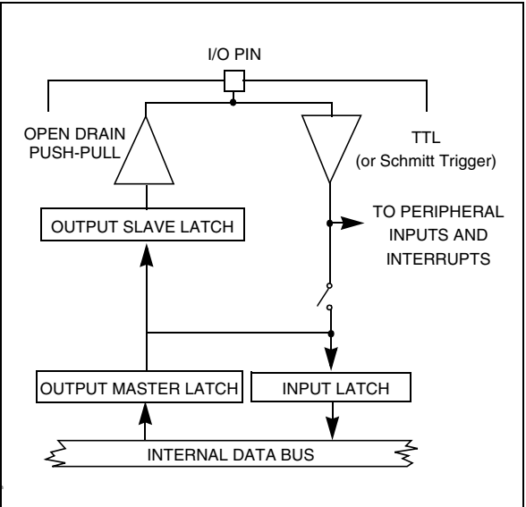
Figure 83. Output Configuration
