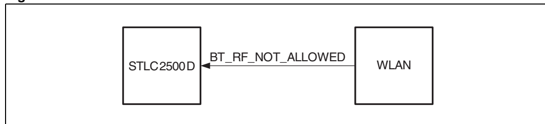
Figure 14. WLAN master
