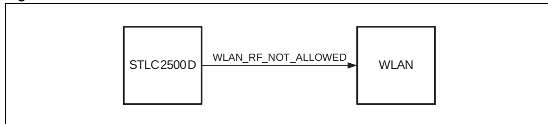
Figure 15. Bluetooth master
