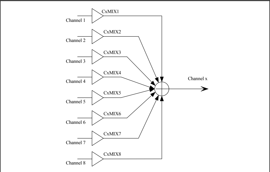
Figure 8. Channel mixer
