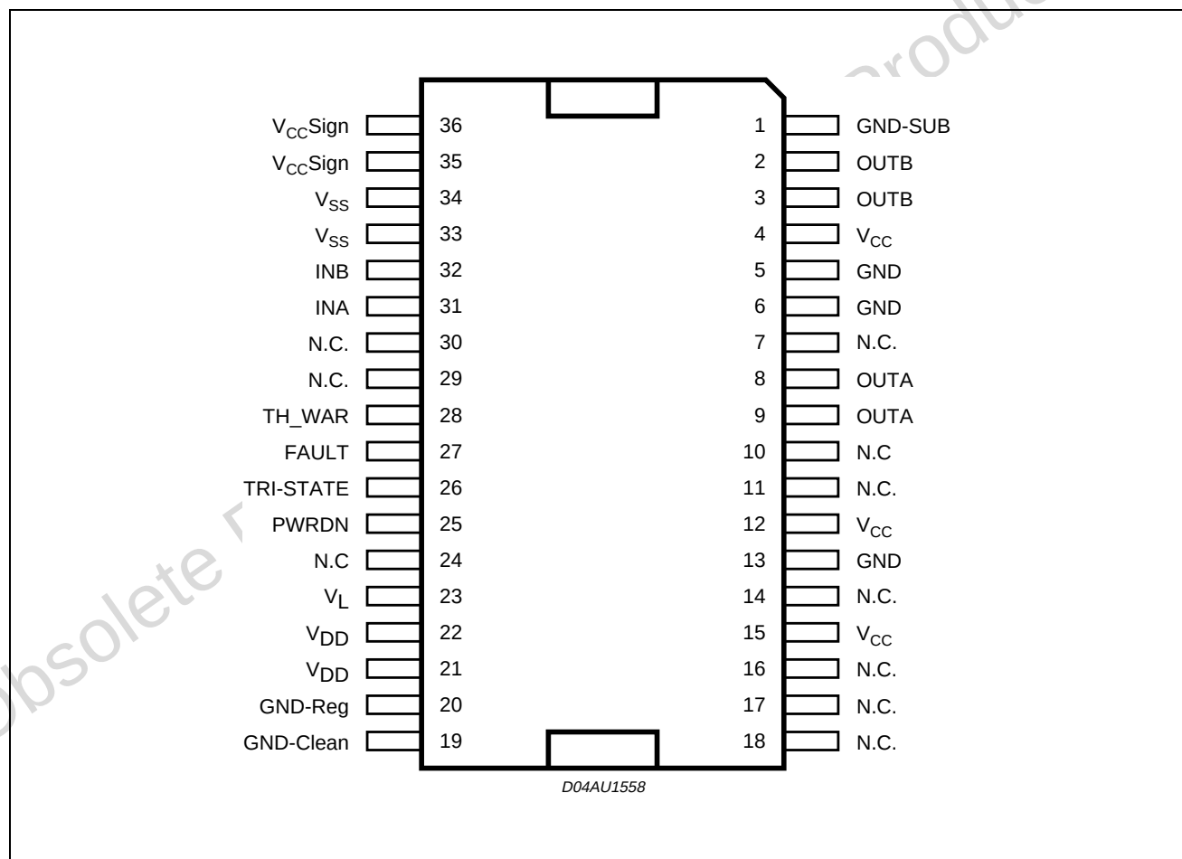
Figure 4. PIN CONNECTION
