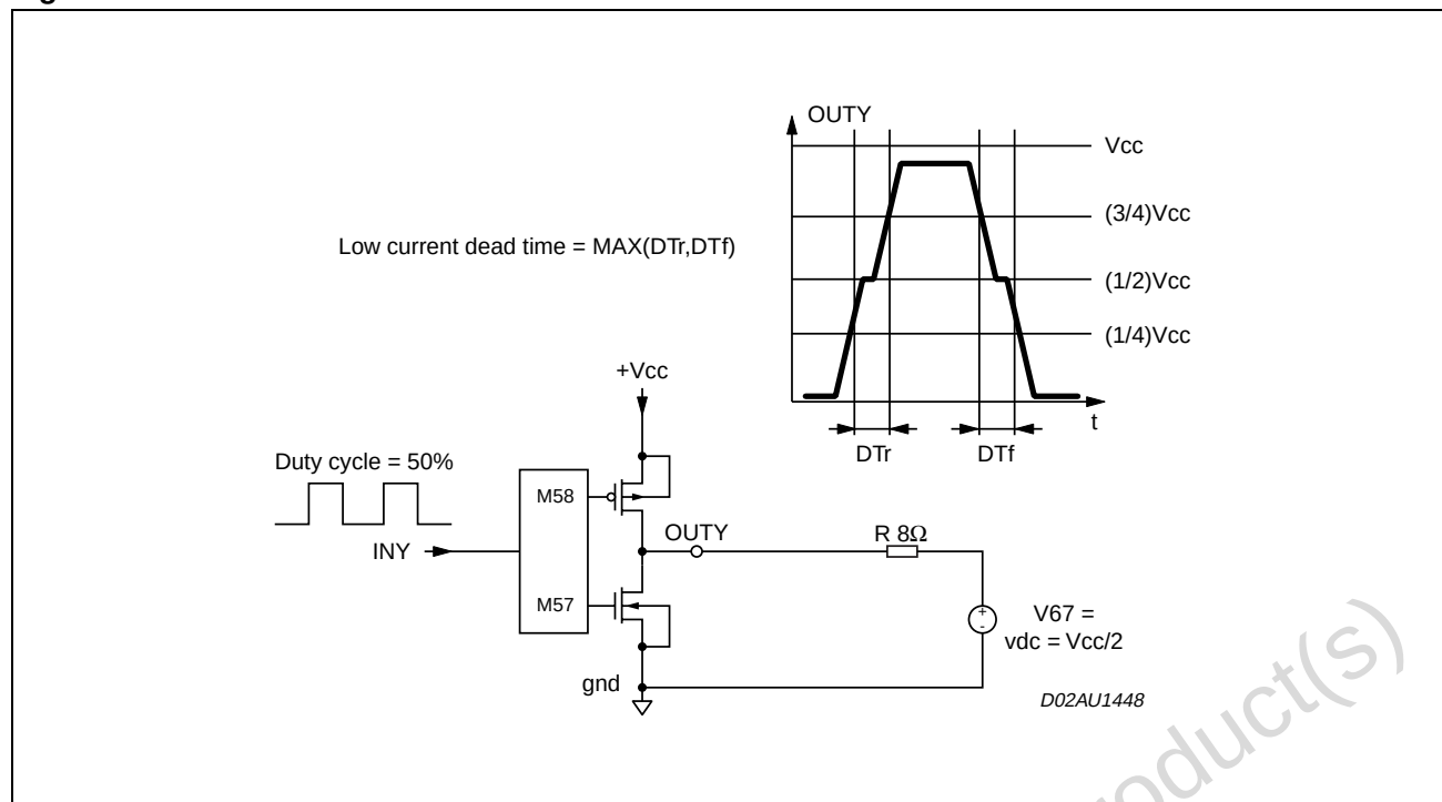
Figure 5. Test Circuit.
