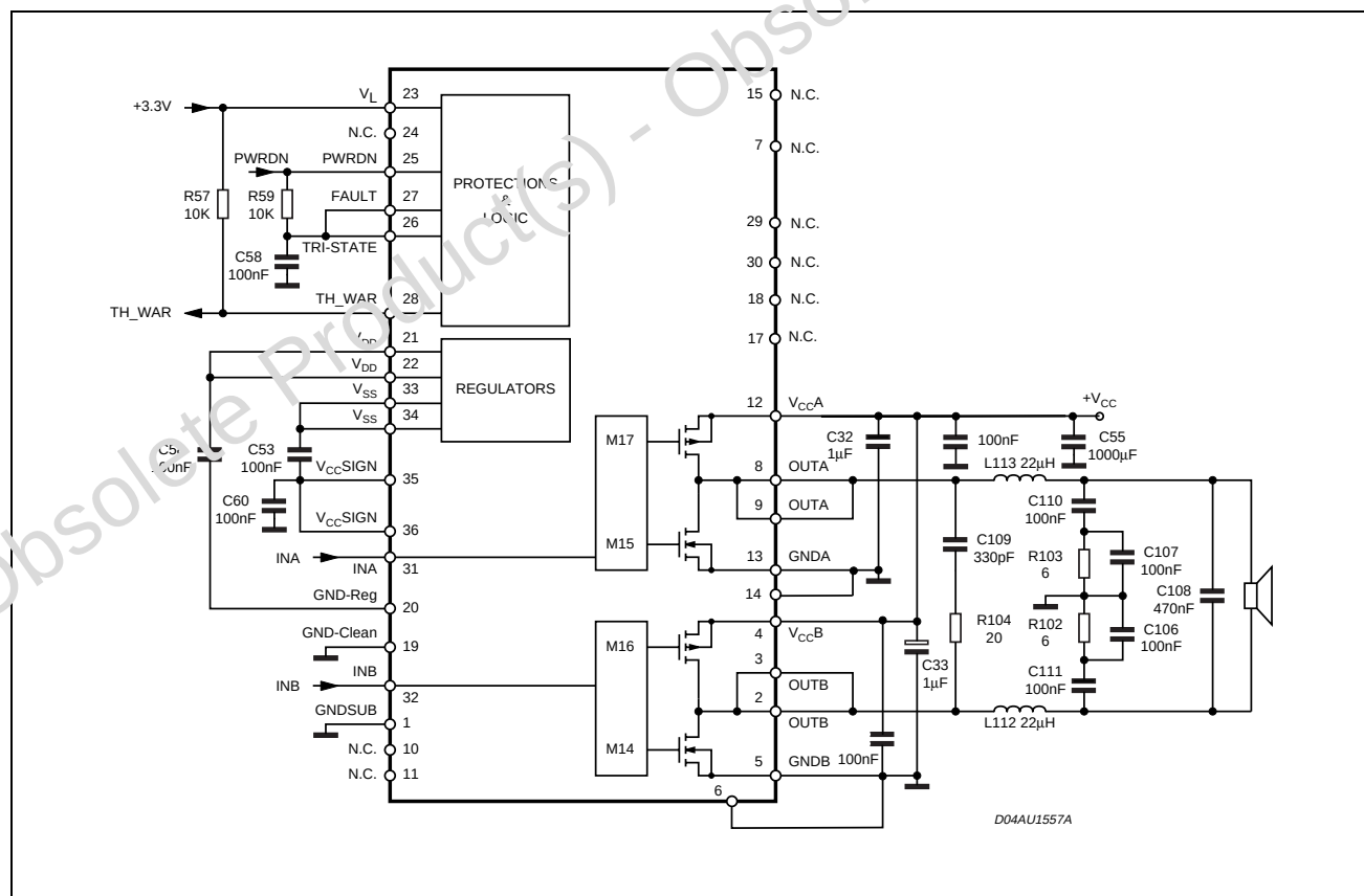
Figure 2. Audio Application Circuit
