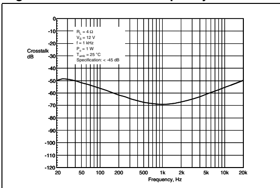
Figure 7. Crosstalk vs frequency
