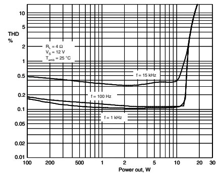
Figure 6. Total harmonic distortion vs output power
