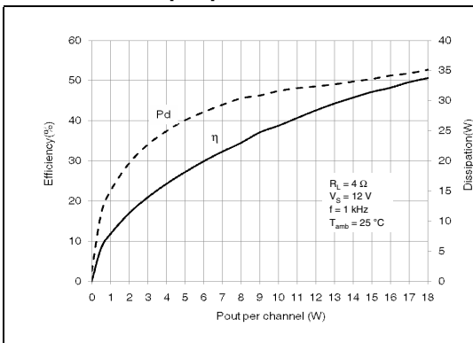
Figure 5. Efficiency, device dissipation vs output power
