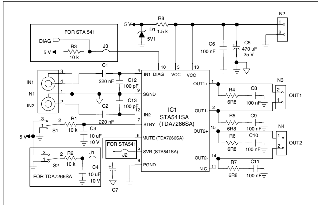
Figure 15. Demo-board schematic
