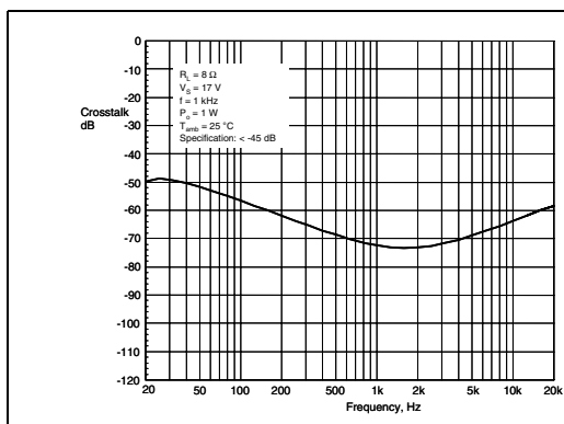
Figure 12. Crosstalk vs frequency
