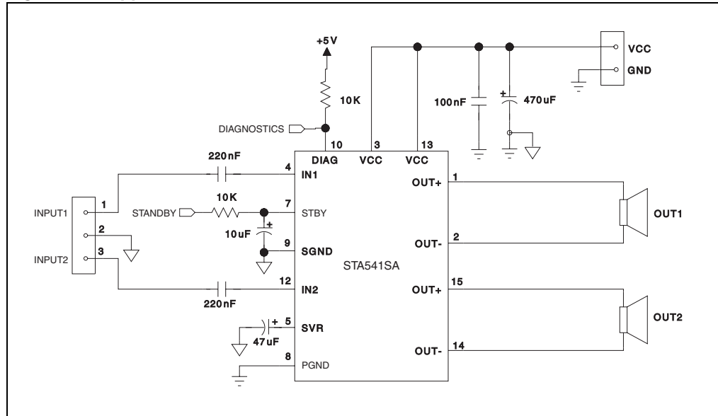
Figure 14. Applications circuit
