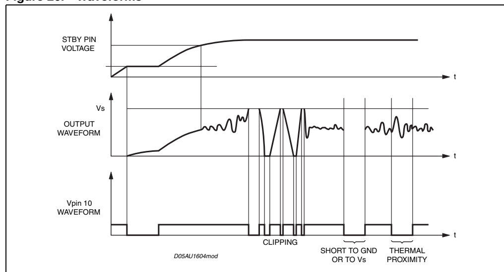
Figure 20. Waveforms
