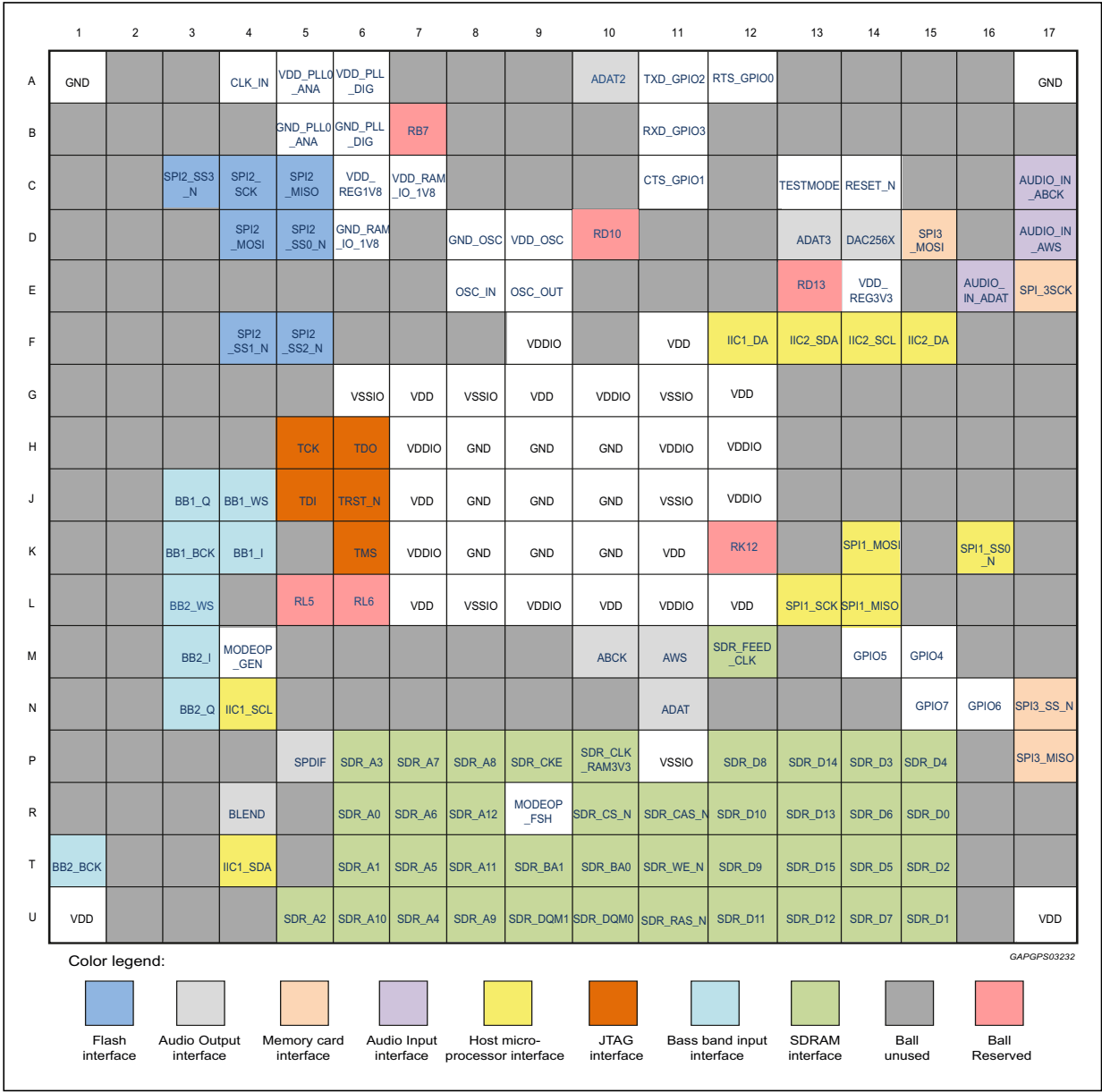
Figure 3. TFBGA ball-out (top view)
