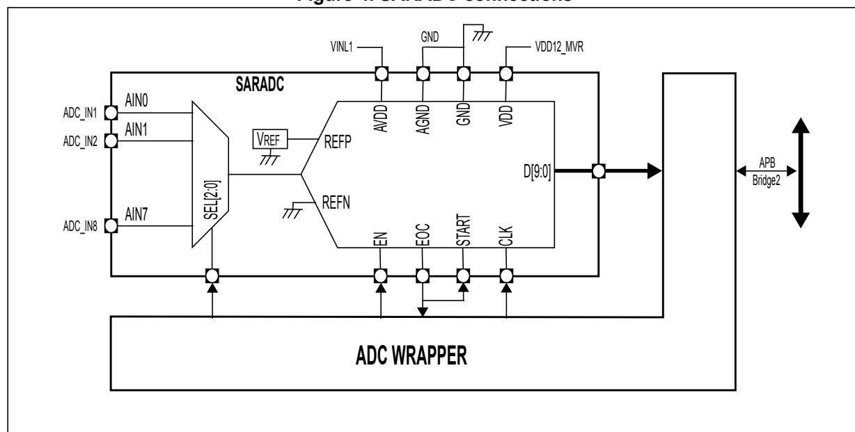
Figure 4. SARADC connections
