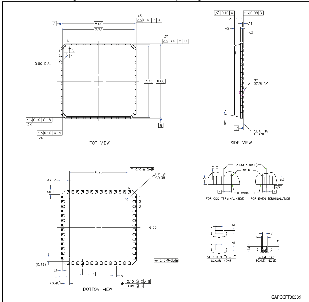
Figure 5. VFQFPN56 8 x 8 mm package dimension
