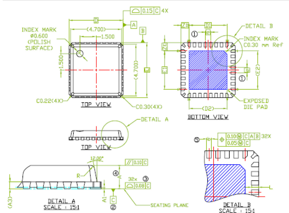
Figure 3. 32-Pad QFN Package Outline and Package Dimensions
