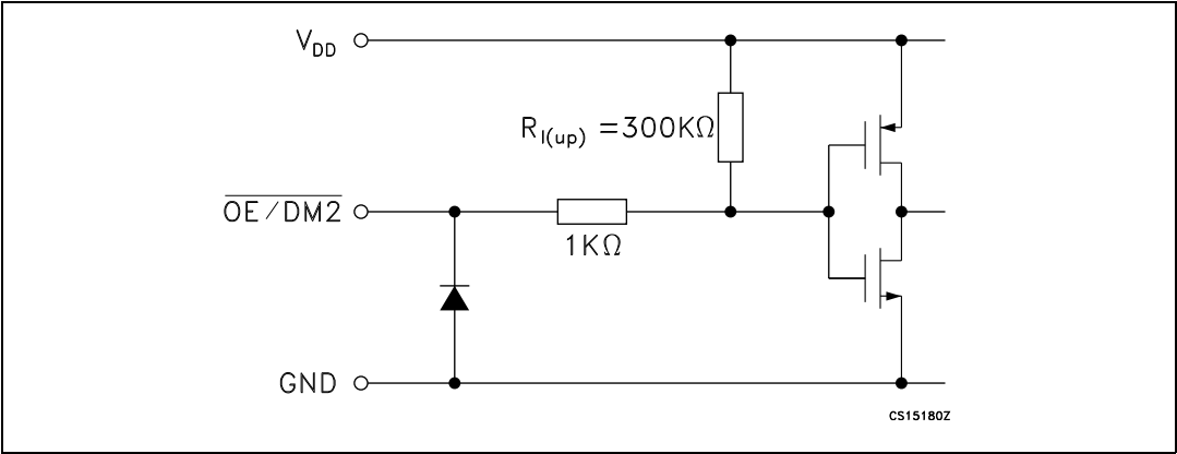
Figure 2. OE/DM2 terminal
