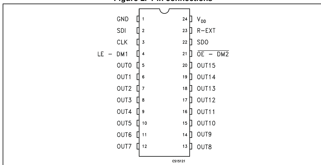
Figure 1. Pin connections
