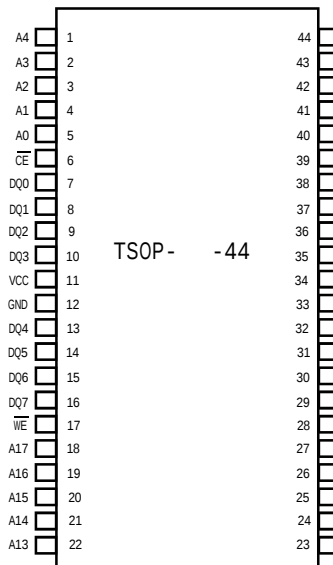
STC62WV25616
