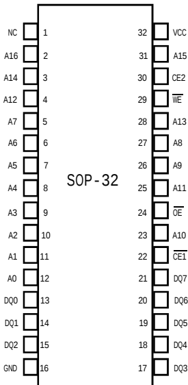
STC62WV25616
