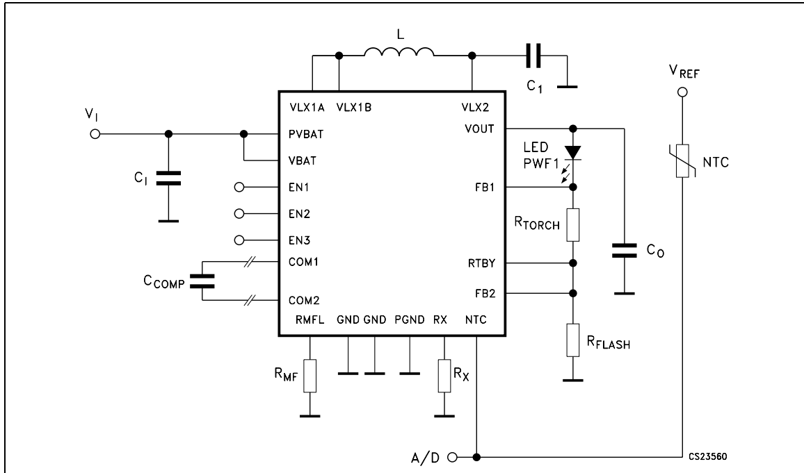
Figure 1. Application circuit
