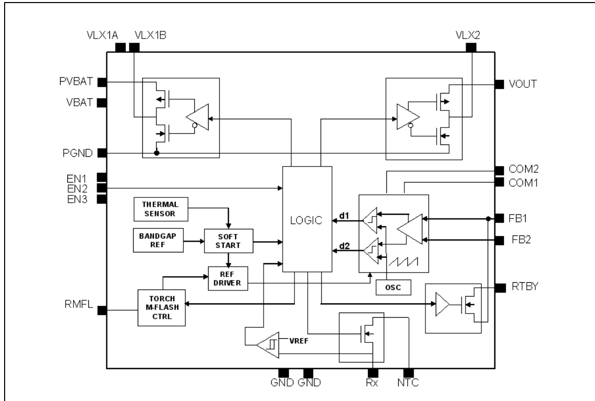
Figure 3. Block diagram
