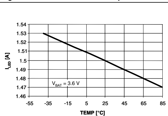
Figure 17. Flash current vs. temperature
