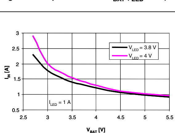
Figure 19. Input current vs. V_{BAT} ( I_{LED} = 1 A)
