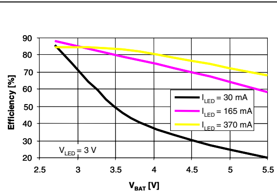
Figure 15. Efficiency vs. V_{BAT} , torch mode
