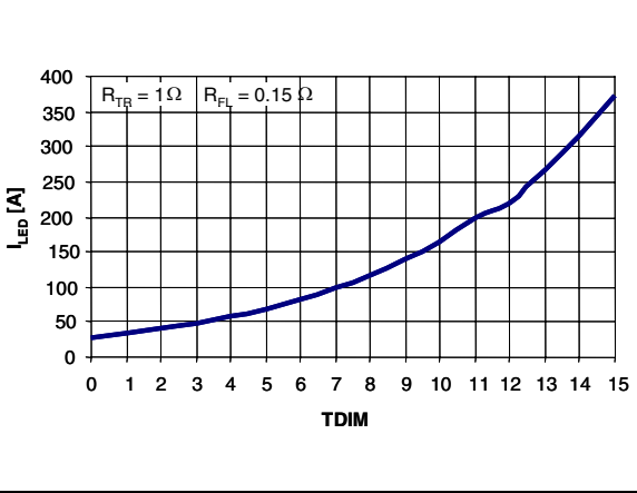
Figure 21. I_{LED} torch vs. TDIM
