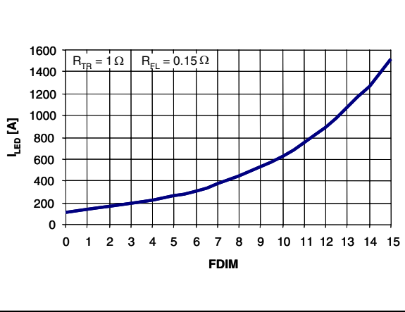
Figure 22. Flash time dimming steps
