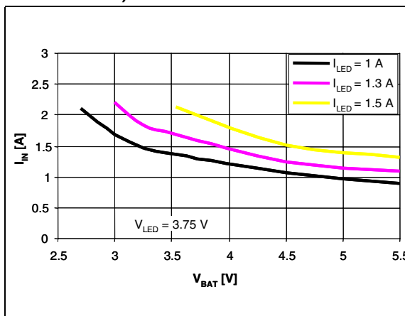
Figure 18. Input current vs. V_{BAT} ( V_{LED} = 3.75 V)
