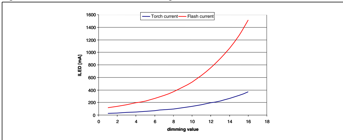
Figure 12. Flash and torch current vs. dimming value
