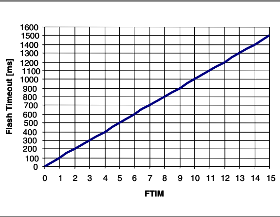
Figure 22. Flash time dimming steps
