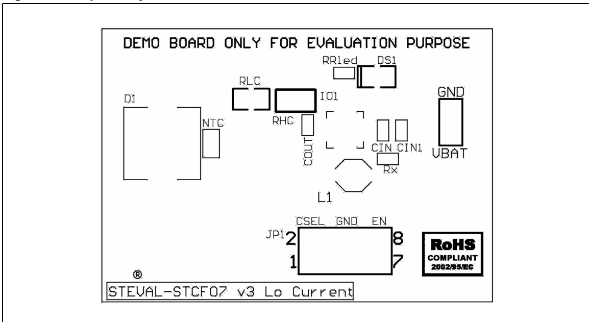
Figure 8. Top overlay
