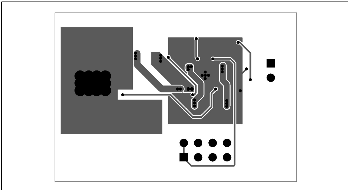
Figure 7. Bottom layer
