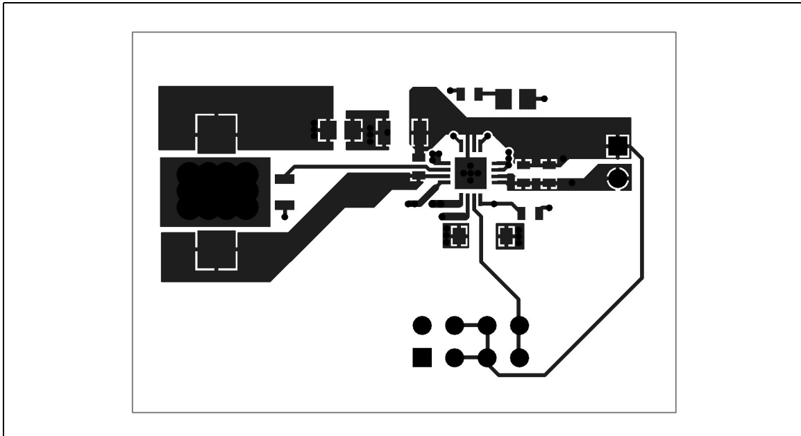
Figure 6. Top layer
