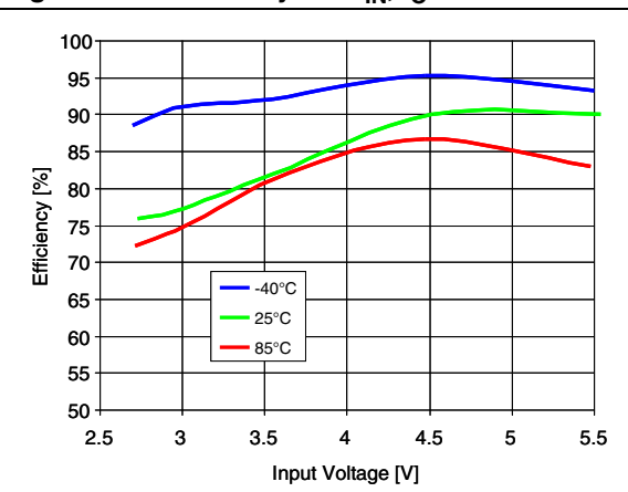
Figure 13. Efficiency vs. V_{IN} , I_O = 400 mA
