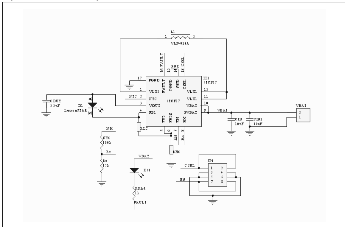
Figure 9. Schematic diagram of the STCF07 demonstration board
