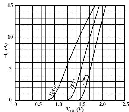
I_C vs. V_{BE} -V_{CE} = 4 \text{ V Continuous}
