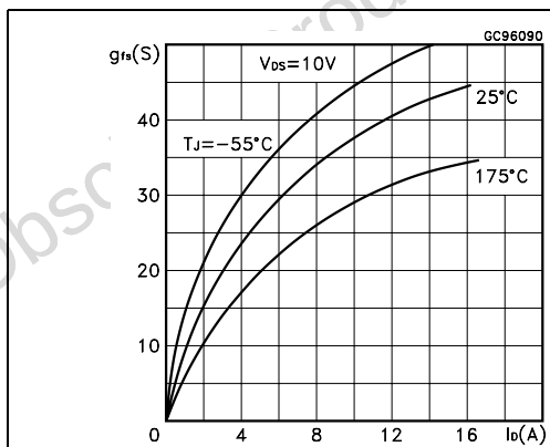
Figure 5. Transconductance
