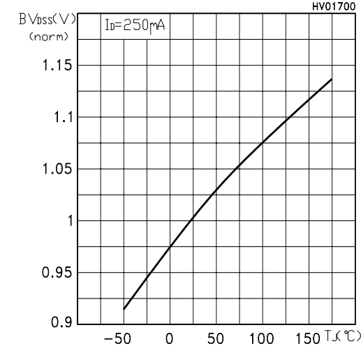
Normalized Drain-Source Breakdown vs Temperature
