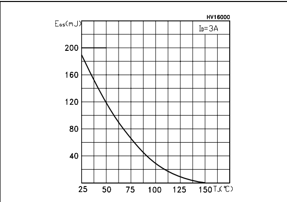
Figure 14. Avalanche energy vs temperature
