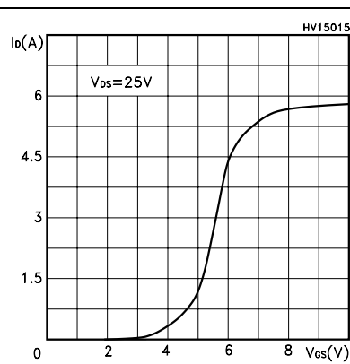
Figure 6. Transfer characteristics
