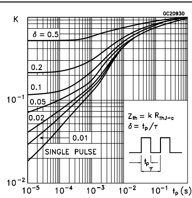
Figure 2. Thermal impedance for TO-220/DPAK/IPAK
