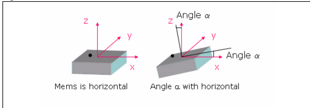
Figure 22. Inclination measurement
