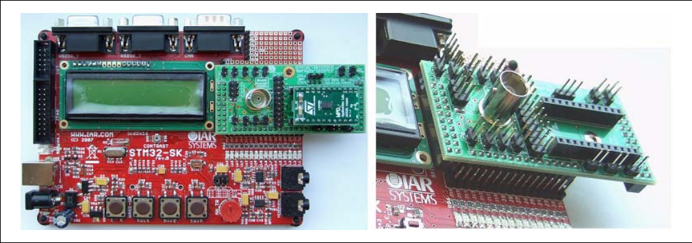
Figure 14. STM3210B-SK/IAR board with STM32-MEMS board connected
