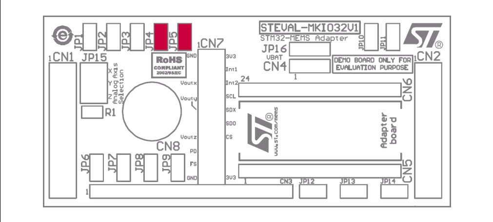
Figure 15. Setup for all MEMS
