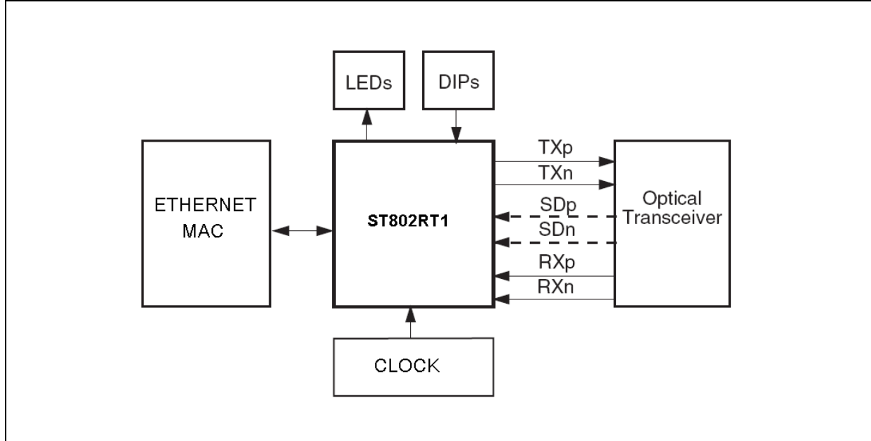
Figure 3. System diagram of the ST802RT1B in FX mode
