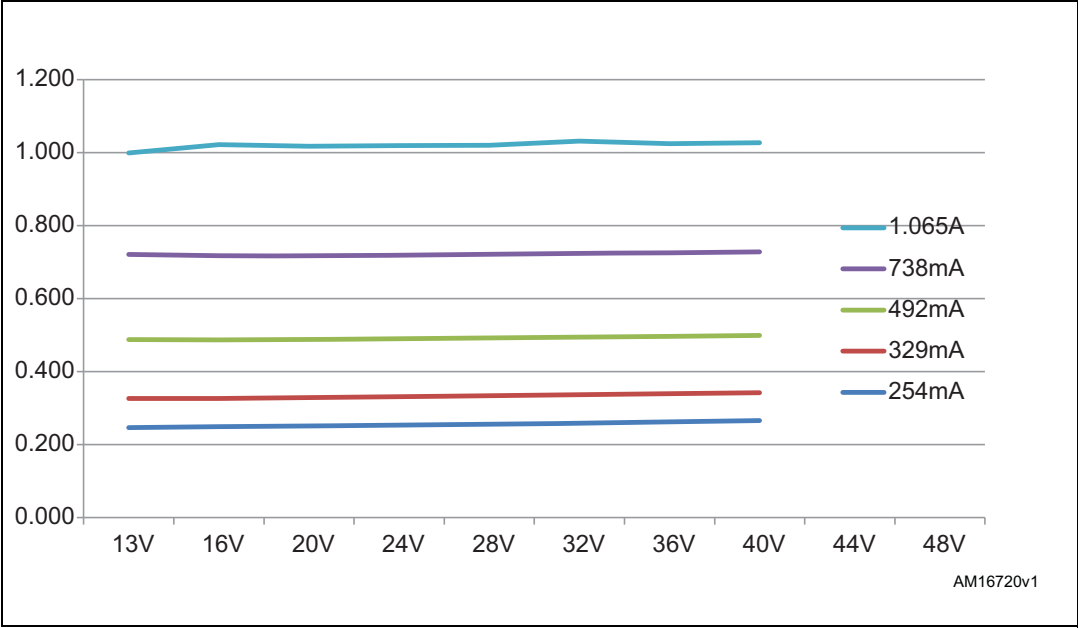
Figure 20. Current regulation vs. V_{PW\_LED} : 3 LEDs
