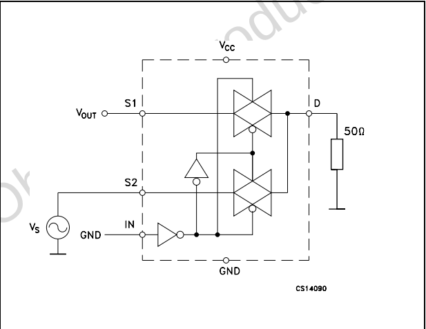
Figure 6. Channel to channel crosstalk
