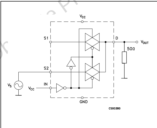
Figure 7. OFF Isolation
