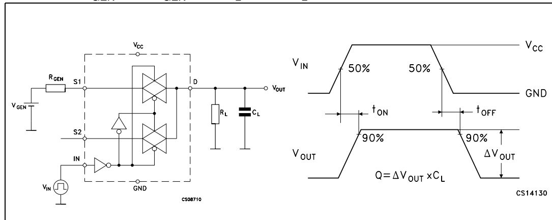
Figure 11. Turn ON, turn OFF delay time
