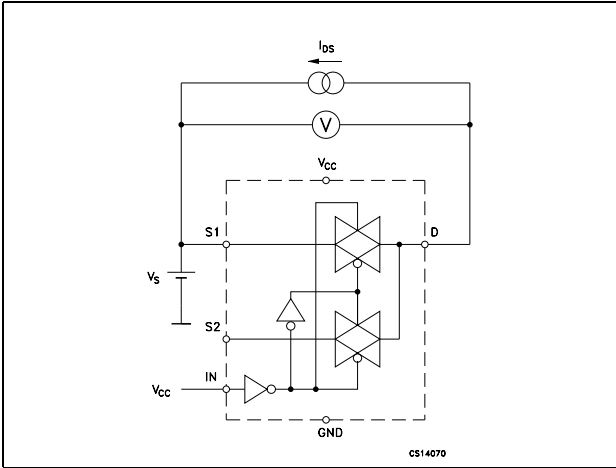
Figure 5. OFF Leakage
