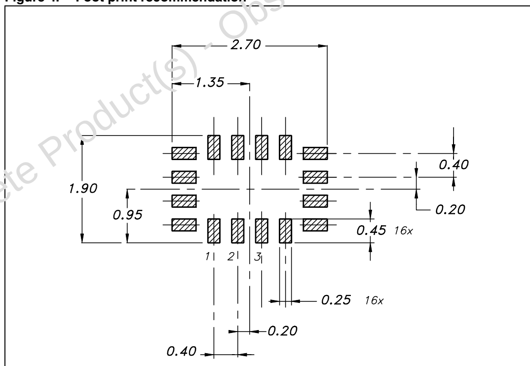
Figure 4. Foot print recommendation
