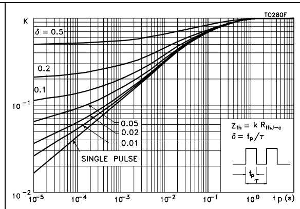
Figure 14. Thermal Impedance
