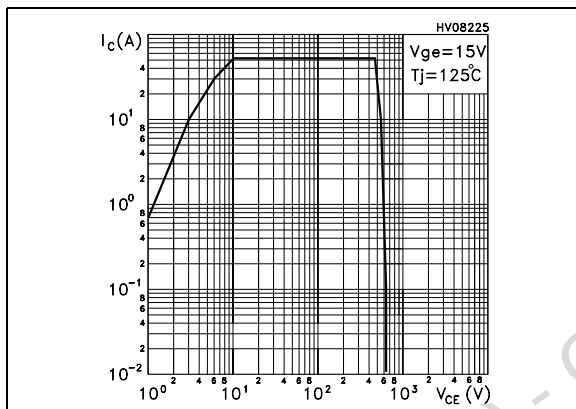
Figure 15. Turn-off SOA
