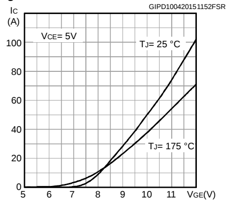
Figure 10: Transfer characteristics
