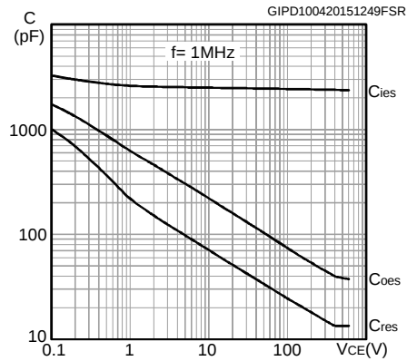
Figure 14: Capacitance variations
