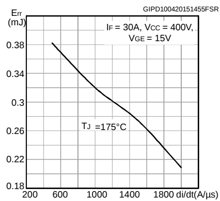
Figure 26: Reverse recovery energy vs. diode current slope
