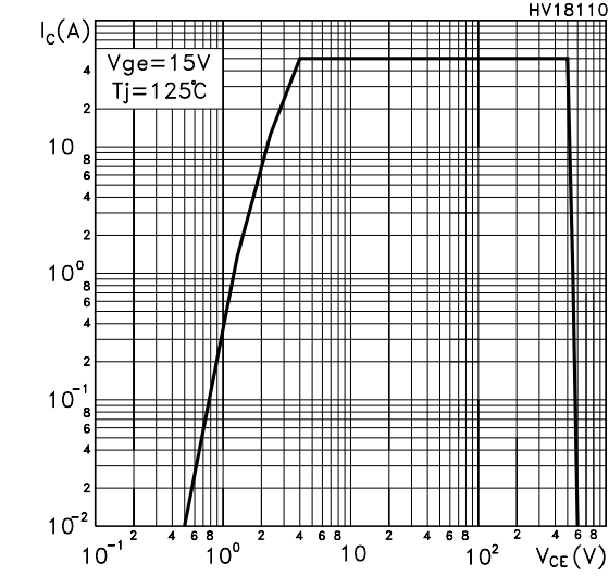
Turn-Off SOA
