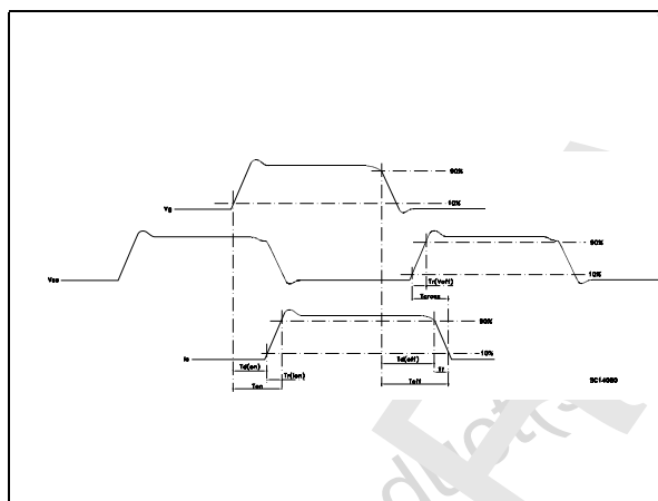
Figure 19. Switching waveforms
