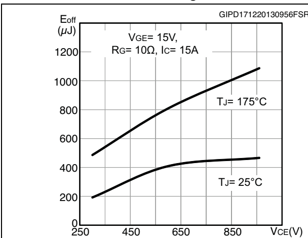
Figure 18. Switching-off loss vs collector-emitter voltage
