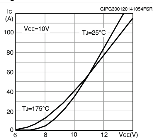
Figure 9. Transfer characteristics
