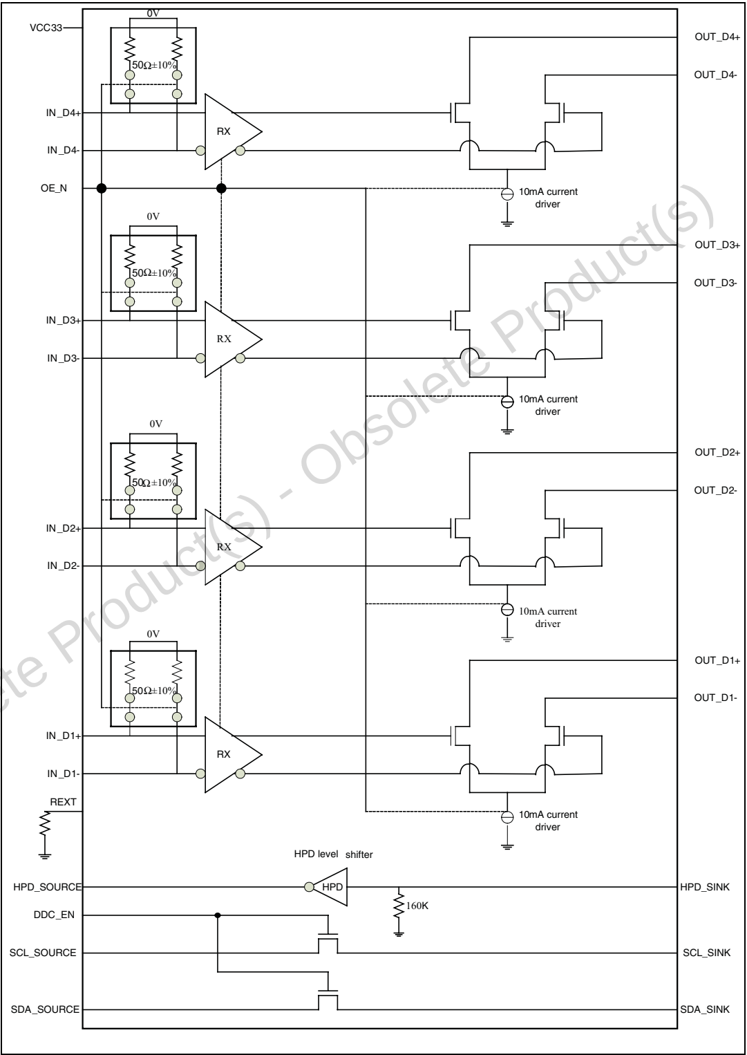
Figure 1. STHDLS101T block diagram
