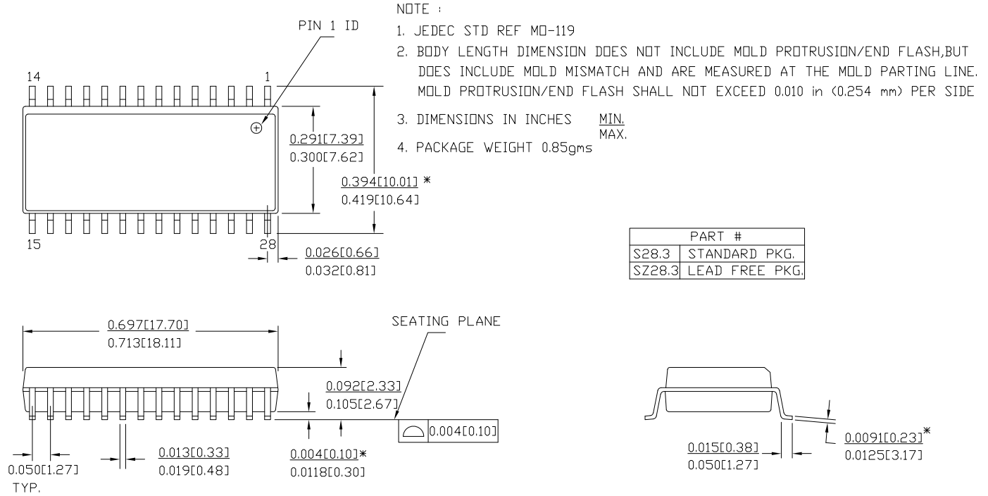
Figure 11. 28-Pin (300 mil) SOIC (51-85026)
