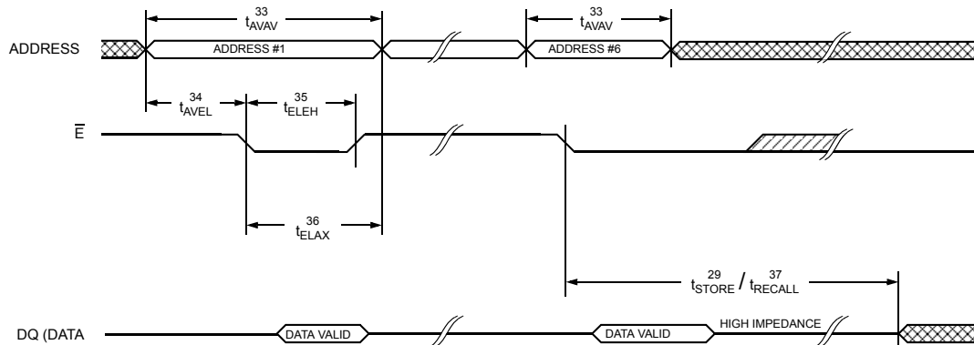
Figure 10. \overline{E} Controlled Software STORE/RECALL Cycle [25]
