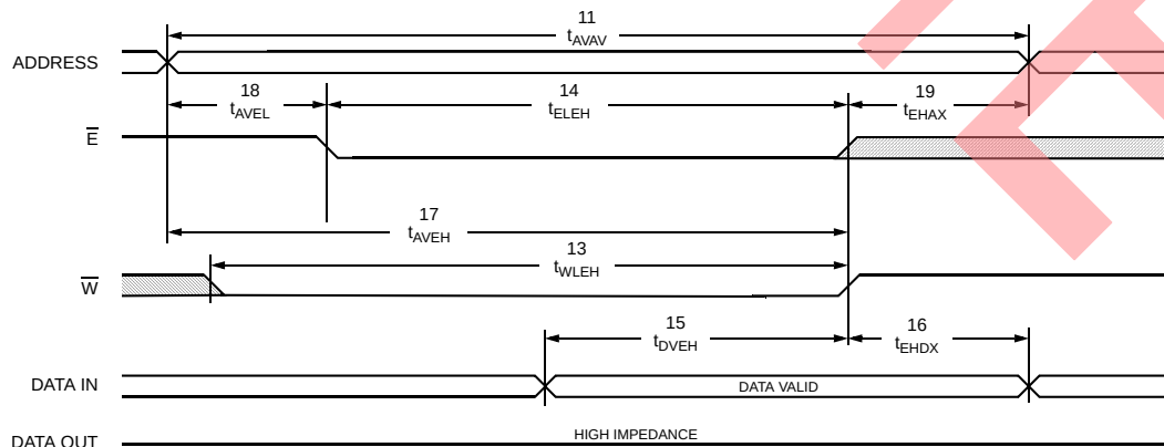
Figure 8. SRAM WRITE Cycle #2: \overline{E} Controlled [8, 9]
