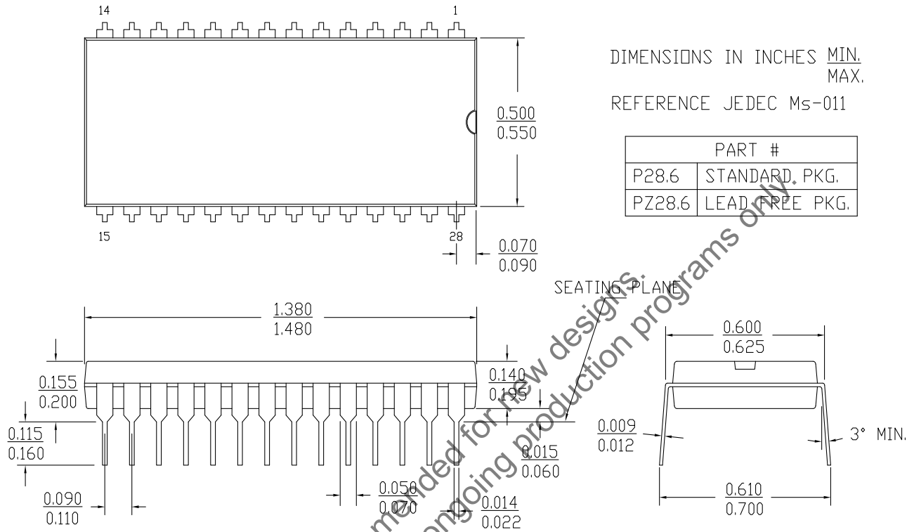
Figure 11. 28-Pin (600 Mil) PDIP (51-85017)
