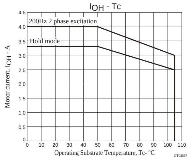
Derating Curve of Motor Current, I_{OH} , vs. STK672-543-E Operating Substrate Temperature, T_c
